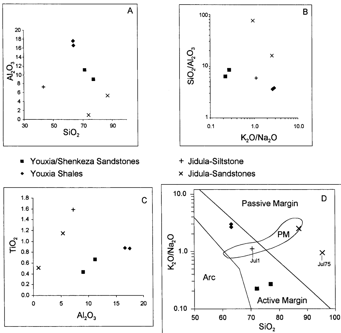
Figure 6. Geochemical plots of the lower Tertiary clastics in the Tingri region. A , Al_2O_3 versus SiO_2 . B , SiO_2/Al_2O_3 versus K_2O/Na_2O . C , TiO_2 versus Al_2O_3 . D , K_2O/Na_2O versus SiO_2 . Tectonic setting fields for D are from Roser and Korsch (1986), with addition of passive margin field from McLennan et al. (1990). In D , Jul 1 and Jul 75 are recalculated to 100% CaO and are volatile free because of significantly high calcite contents.
