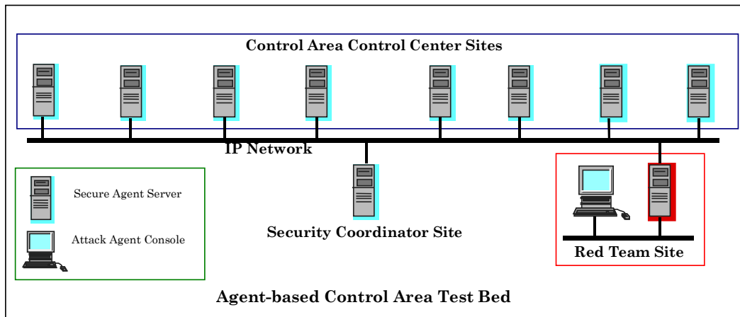
Figure 1. Proposed Control Area / Security Coordinator Test Bed
