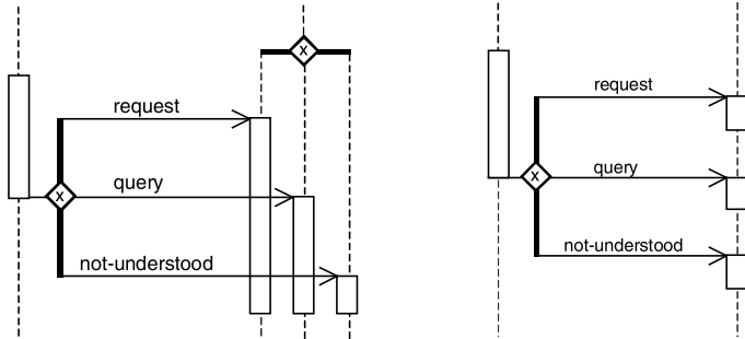
Figure 3. Full and abbreviated notation of XOR connection
