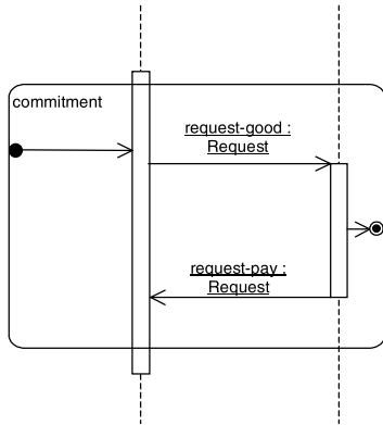
Figure 5. Input/output of nested protocols
