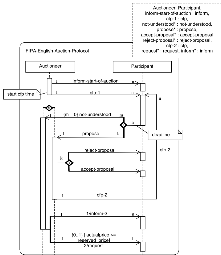
Figure 6. A generic AIP expressed as a template
