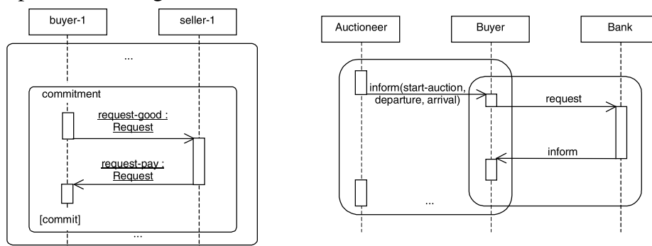
Figure 4. nested protocol and interleaved protocol
