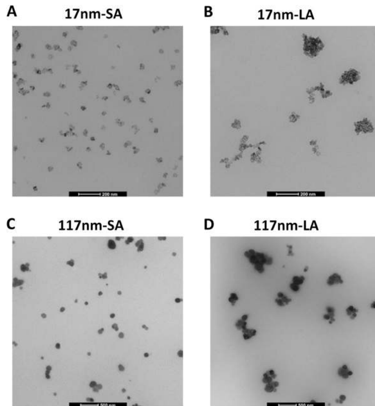
Fig. 1 Representative TEM micrographs of freshly prepared TiO 2 stock suspensions of small (SA) and large agglomerates (LA). 17 nm-SA (a), 17 nm-LA (b), 117 nm-SA (c) and 117 nm-LA (d)
