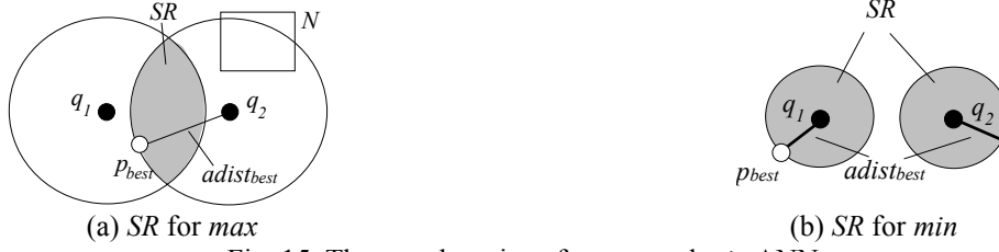
Fig. 15. The search regions for max and min ANN
