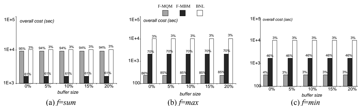
Fig. 48. Overall cost vs. buffer size ( P=LA , Q=TS , k=4 , A_Q=8\% )
