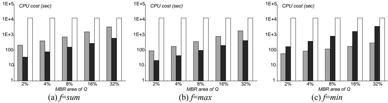
Fig. 43. CPU cost vs. area A_Q of Q ( P=TS , Q=LA , k=4 )
