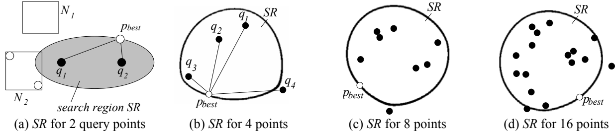
Fig. 14. The search regions for sum ANN
