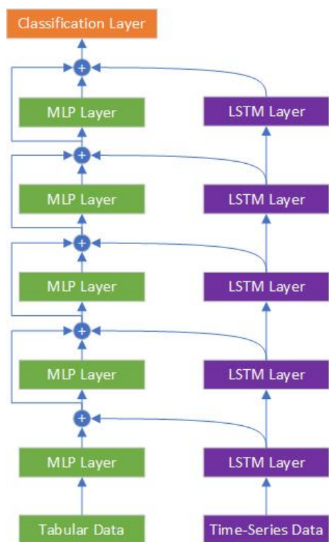
FIGURE 2. The proposed MLP-LSTM architecture.
