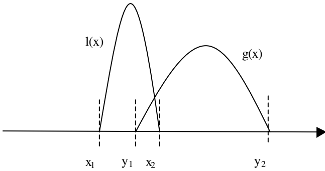
Figure 4. Bounded distributions
