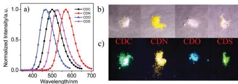
Fig. 3 (a) The normalized emission spectra of CDC, CDN, CDO and CDS in the solid state, \lambda_{\text{ex}} = 300 nm for CDC and CDO, \lambda_{\text{ex}} = 330 nm for CDN and CDS. (b) Photos of compounds CDC, CDN, CDO and CDS as solid powders under room light and (c) fluorescence images under UV illumination (365 nm), 20 °C.
