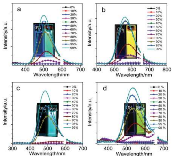
Fig. 2 Fluorescence spectra of (a) CDC, (b) CDN, (c) CDO and (d) CDS in THF/water mixtures with different water volume fractions; \lambda_{\text{ex}} = 300 nm for CDC and CDO, \lambda_{\text{ex}} = 330 nm for CDN and CDS, c = 5.0 \times 10^{-5} M, 20 °C (light scattering from the incident light was omitted in the spectra).
