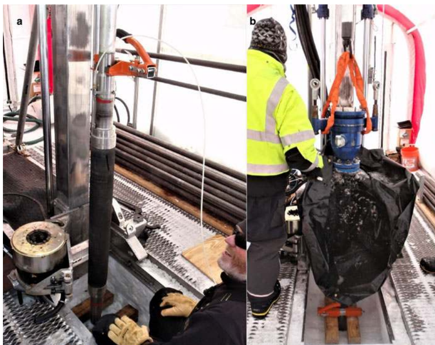
Fig. 4. (a) Inflatable packer installation. (b) Diverter and sump pit liner installation.
