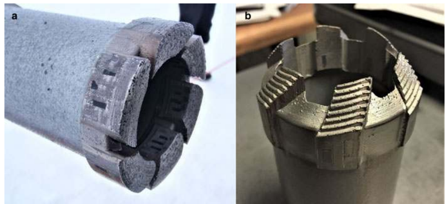
Fig. 6. (a) Worn diamond-impregnated coring bit for rock. (b) Hybrid diamond-impregnated coring bit, designed to core through the ice-rock transition, have been mostly unsuccessful due to the excessive pump pressure required.
