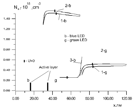
Figure 4. Distribution of the effective charged centers concentration on the p-side of the space charge region of blue (b) and green (g) LED's before and after aging at J = 80 mA: 1) t=0 ; 2) t=250 hours; 3) t=1000 hours.
