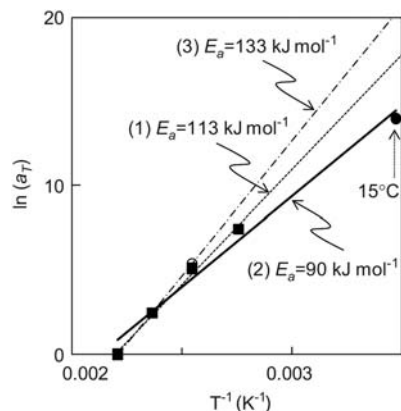
Figure 4 Arrhenius plots of shift factors from empirical superposition of the change of \Delta E^*_{ab} , regression lines, and apparent activation energies for the plots of (1) heat treated wood, (2) heat treated wood and naturally aging wood, and (3) heat treated naturally aging wood (■: heat treated, ●: natural aging, ○: heat treated after natural aging).
