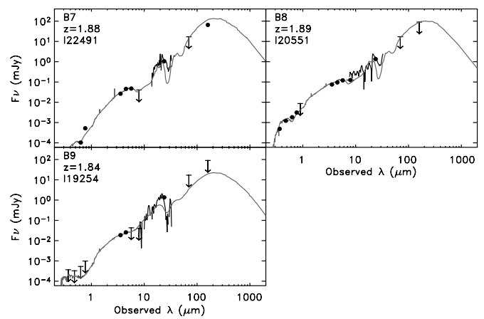
FIG. 8.—Same as Fig. 5, but for overall SEDs of starburst sources B7–B9. Jagged curves : IRS spectra from Fig. 4.
