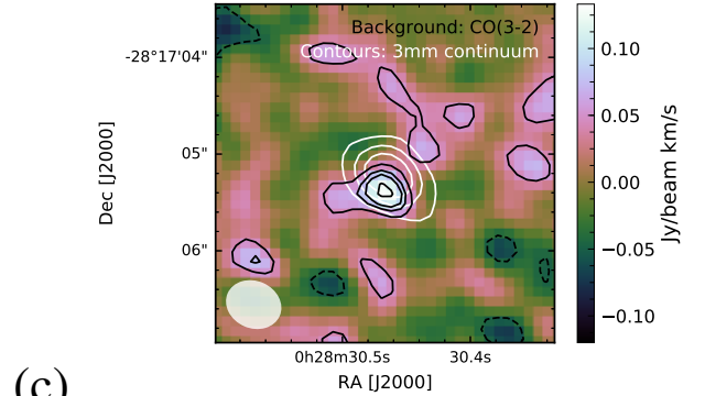
Fig. 4. 2QZJ0028 : (a) White contours show the continuum emission from 2QZJ0028 at 3 mm with a beam of 0.64'' \times 0.53'' . Contours are at the level of 3, 5 and 7 times the noise per beam ( 12 \mu\text{Jy} ). The color background image shows the continuum emission in H-band from SINFONI data of 2QZJ0028. (b) ALMA spectrum extracted from an aperture as large as the beam size and rebinned to 60 km/s. The vertical dashed green line mark the expected positions for CO(3-2) emission line at the redshifted of the narrow H \alpha component (Cano-Díaz et al. 2012): the line is not detected. An emission line is detected at a velocity of \sim -2000 km/s with respect to the redshift of 2QZJ0028. (c) CO(3-2) surface brightness. Black solid contours are at the levels of 2\sigma , 3\sigma , 4\sigma and 5\sigma , where \sigma is 0.03 \text{ Jy/beam km/s} . The white contours show the continuum emission at 3 mm at the levels of 3, 6, and 9 times the sensitivity of the continuum map. The synthesised beam is shown in the bottom-left corner.
