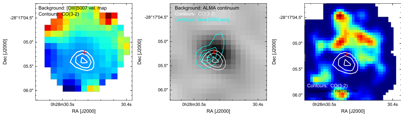
Fig. 5. 2QZJ0028: from left to right: [OIII] \lambda 5007 velocity map by Carniani et al. 2015b, ALMA continuum map at 3 mm, and narrow H \alpha emission tracing SF in the host galaxy (Cano-Díaz et al. 2012). White contours trace the flux map of CO(3-2) emission at the same levels of the levels 3, 4 and 5\sigma . The red cross indicates the centroid of the H-band continuum emission. The cyan contours in the middle panel shows the flux map of the blue [OIII] \lambda 5007 wings collapsing the SINFONI cube over the velocity range -2500 < v < -2300 km/s.
