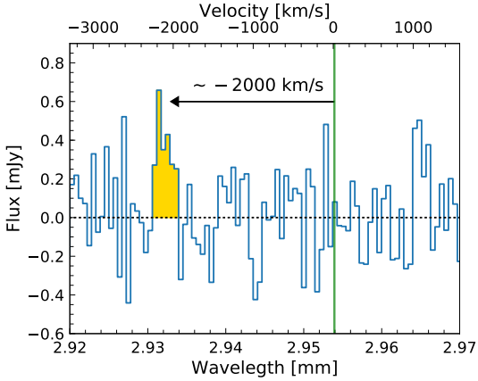
Fig. 4. 2QZJ0028 : (a) White contours show the continuum emission from 2QZJ0028 at 3 mm with a beam of 0.64'' \times 0.53'' . Contours are at the level of 3, 5 and 7 times the noise per beam ( 12 \mu\text{Jy} ). The color background image shows the continuum emission in H-band from SINFONI data of 2QZJ0028. (b) ALMA spectrum extracted from an aperture as large as the beam size and rebinned to 60 km/s. The vertical dashed green line mark the expected positions for CO(3-2) emission line at the redshifted of the narrow H \alpha component (Cano-Díaz et al. 2012): the line is not detected. An emission line is detected at a velocity of \sim -2000 km/s with respect to the redshift of 2QZJ0028. (c) CO(3-2) surface brightness. Black solid contours are at the levels of 2\sigma , 3\sigma , 4\sigma and 5\sigma , where \sigma is 0.03 \text{ Jy/beam km/s} . The white contours show the continuum emission at 3 mm at the levels of 3, 6, and 9 times the sensitivity of the continuum map. The synthesised beam is shown in the bottom-left corner.
