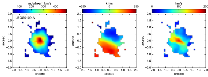
Fig. A.4. CO(3-2) flux, median velocity, and velocity dispersion maps of LBQS0109-A. The maps are obtained by selecting pixel with S/N > 3 . The velocity map shows a gradient of velocity towards the north-south direction.
