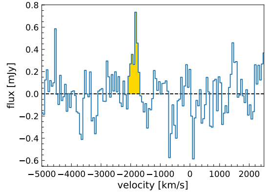
Fig. B.1. ALMA spectrum extracted from the emission peak of the line detection, spatially offset by 0.2'' relative to the location of 2QZJ0028. The spectrum is rebinned to 60 km/s.
