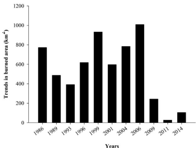
Figure 5. Trends in burned area extent in the upper Teles Pires River basin, Brazil, from 1986-2014.
