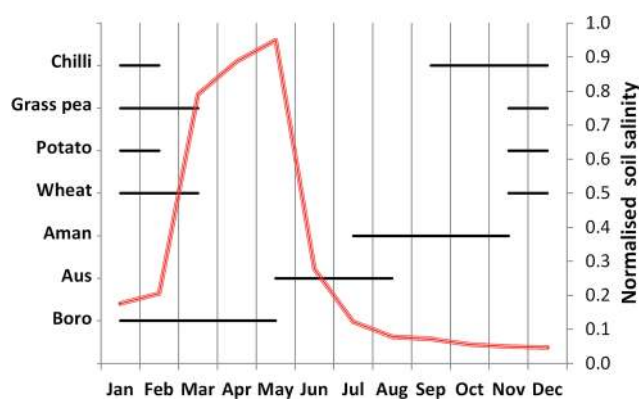
Fig. 7 Salinity (red line) only affects the growth period (black horizontal lines) of a few crops.
