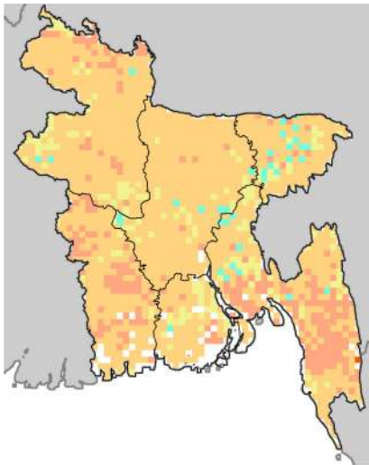
c. ECHAM
