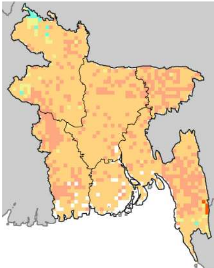
c. ECHAM
