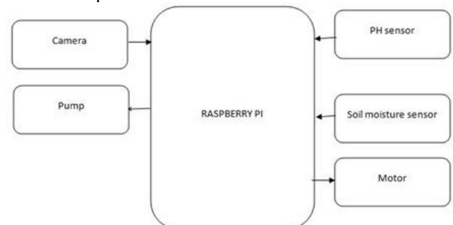
Fig.1 Block Diagram of Raspberry pi
