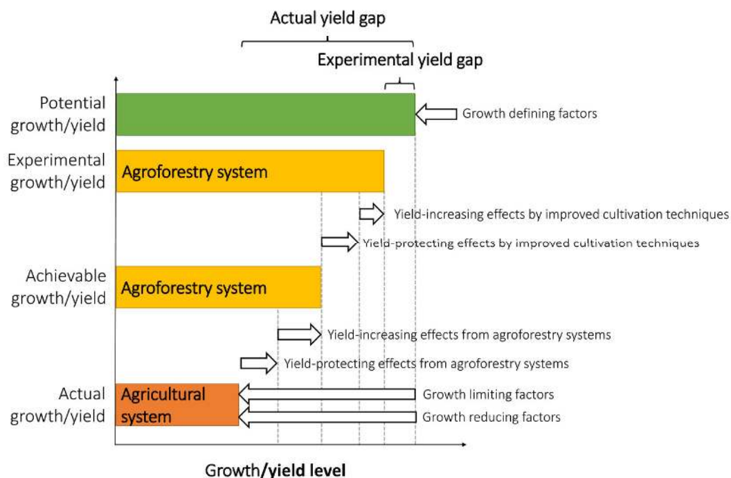
Figure 4. Yield potentials and yield gaps and relationships among yield levels and growth-defining, growth-limiting and growth-reducing factors, and yield-increasing and yield-protecting measures (after [221]).
