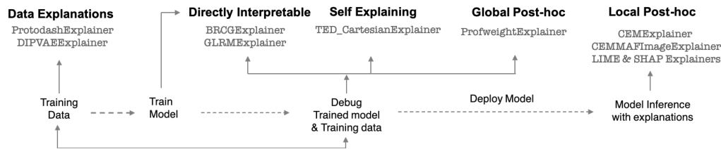
Figure 2: AIX360 class structure organized according to use in the AI pipeline.
