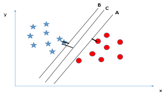
FIGURE 5. SVM illustration.
