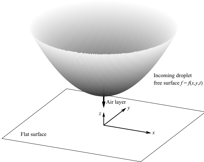
FIGURE 1. An initially spherical droplet approaches impact with a flat surface. The impact is cushioned by the air in the gap between the droplet and the solid.
