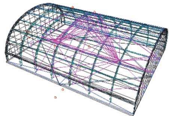
Figure 12: 3D air dome virtual model with the indication of the sound reflection under the vault
