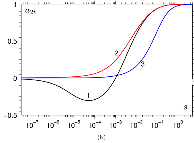
Figure 6: Tangential velocities as a function of distance from the contact line s along the (a) liquid-gas and (b) gas-solid boundaries computed at Ca = 0.4 with curve 1: (\bar{P}_g, A) = (0.14, 0) , 2: (0.14, 1) and 3: (0.014, 1) . The velocity tangential to the free-surface and pointing towards the contact line is u_{1t} , with subscripts ‘a’ for the liquid-facing side of the interface and subscripts ‘b’ for the gas side. The tangential velocity on the gas-solid interface pointing towards the contact line is u_{2t} and the speed of the solid is 1.
