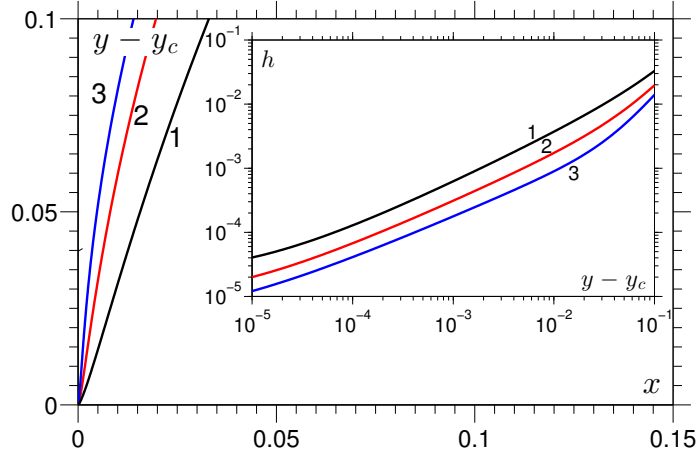
Figure 7: Free-surface shapes obtained in our base case, with \bar{P}_g = 0.014 , with curve 1: Ca = 0.4 (in black), 2: Ca = 0.6 (in red) and 3: Ca = 0.8 (in blue). The inset shows how the height of the gas film h varies as a function of y - y_c showing that for 10^{-4} < y - y_c < 10^{-1} it can be considered in a lubrication setting.
