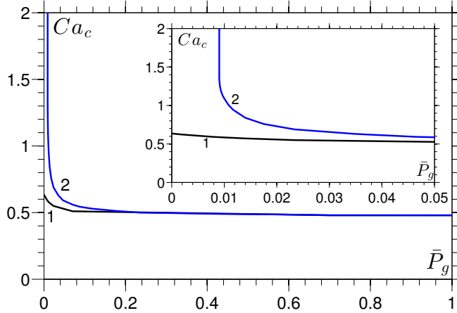
Figure 4: The dependence of the critical capillary number Ca_c on the gas pressure \bar{P}_g , for our base parameters, with curve 1: A = 0 (in black) and 2: A = 1 (in blue). The inset shows how curve 1 ( A = 0 ) tends to a finite value of Ca_c as \bar{P}_g \rightarrow 0 whilst curve 2 appear to increase without bound.
