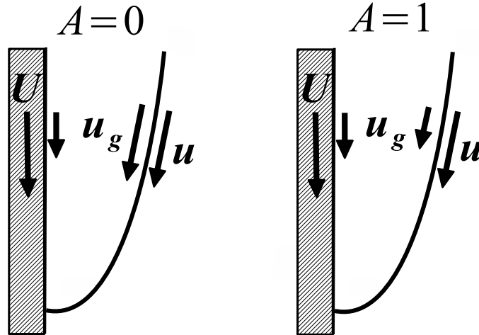
Figure 3: The effect of Maxwell-slip on the gas flow. When A = 0 slip is present at the gas-solid boundary but turned off at the gas-liquid boundary, so that \mathbf{u}_g = \mathbf{u}_g , whilst for A = 1 it is present on both interfaces.
