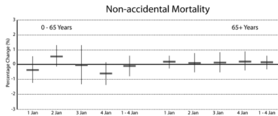
Figure 3. Mean percent increase (95% CI) in daily non-accidental mortality for 0–65 years and over 65 years associated with 10\mu\text{g}/\text{m}^3 PM 10 concentration on 1 January 0–6 hours.
