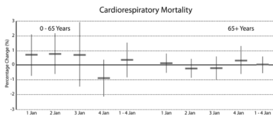
Figure 4. Mean percent increase (95% CI) in daily cardiorespiratory mortality for 0–65 years and over 65 years associated with 10\mu\text{g}/\text{m}^3 PM 10 concentration on 1 January 0–6 hours.
