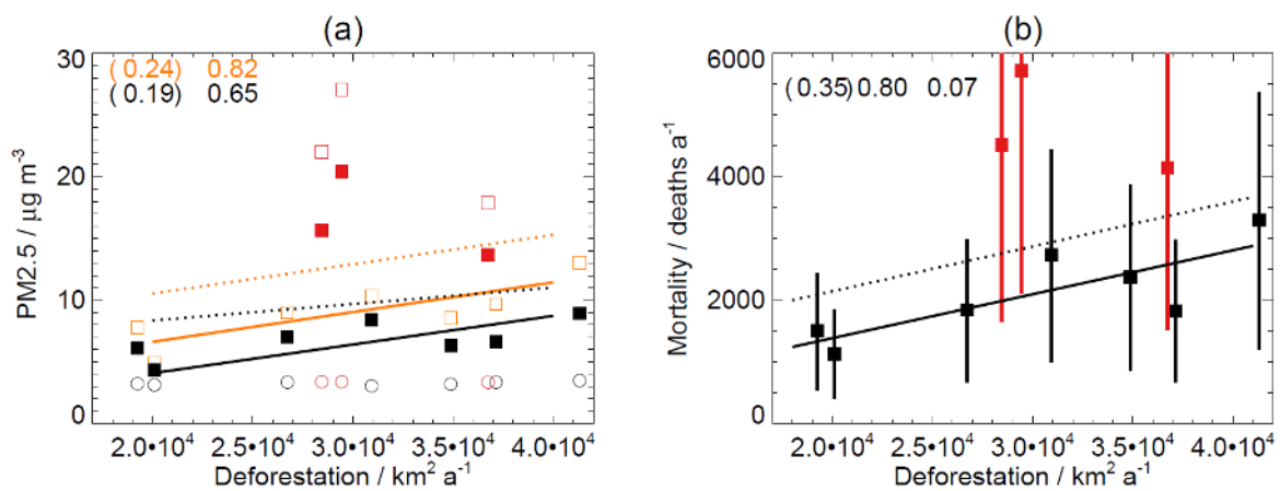
Figure 3. Relationship between Brazil's deforestation rates, simulated PM2.5 and premature mortality. (a) Simulated regional (50°-70°W, 5°-25°S) dry season surface PM2.5 concentrations against Brazil's deforestation rates (black filled square: deforestation fires, orange open square: all fire, circles: without fire). (b) Simulated annual mortality in South America due to exposure to PM2.5 from deforestation fires (error bars show 95% confidence interval) against Brazil's deforestation rates. Drought years indicated in red. Lines show linear relationship (solid: excludes drought, dashed: all years) with Pearson's linear correlation coefficient (r) detailed on each panel (value for all years in parenthesis) and gradient of best-fit line (b).
