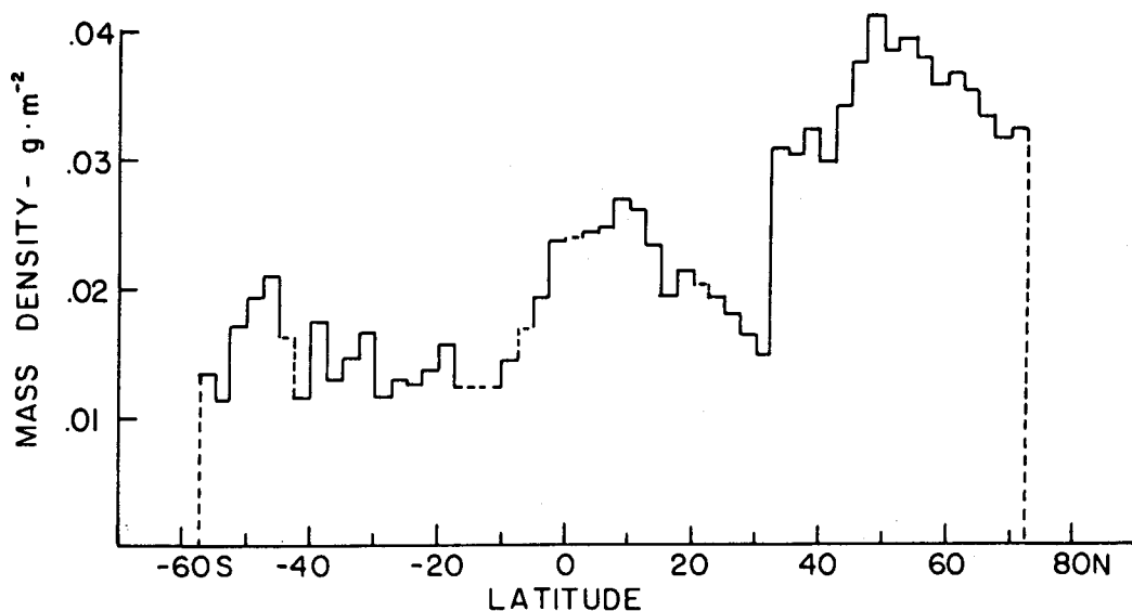
Fig. 24. Column mass density for the data in Figure 23.
