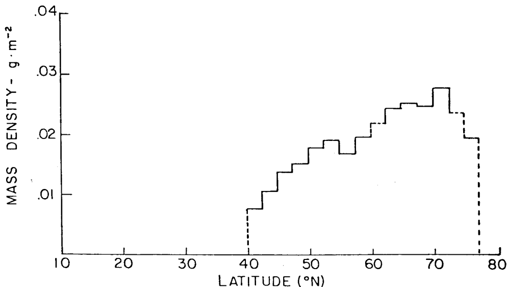
Fig. 25. Column mass density versus latitude for the survey flight of January 1984. Data have been averaged into 2.5^\circ latitude bins.
