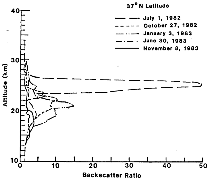
Fig. 4. Lidar profiles of backscatter ratio (R) at \lambda = 0.6943 \mu\text{m} versus altitude for ground-based data taken at 37^\circ\text{N} , 76^\circ\text{W} .
