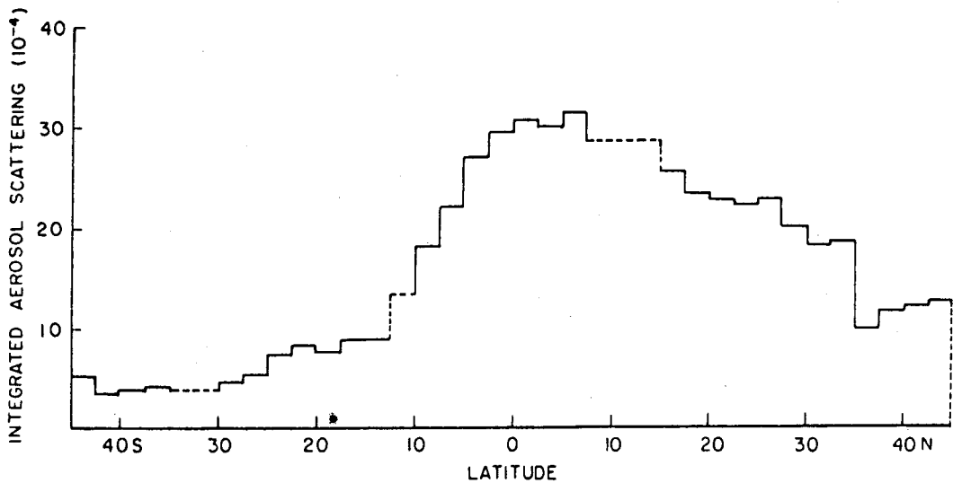
Fig. 13. Integrated scattering function from Figure 12 but averaged into 2.5^\circ latitude bins for both flight legs.
