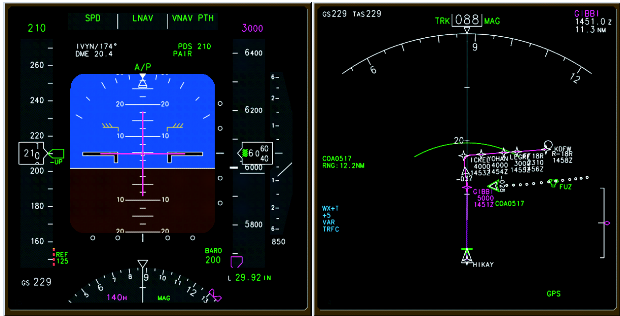
Fig. 5 Primary Flight Display (PFD) and Navigation Display (ND) of the Boeing 777-like simulator with AMSTAR/Pair Dependent Spacing symbology. The PFD shows the PDS annunciation in the upper right corner under the Flight Mode Annunciator and the commanded speed on the speed tape. The ND shows the lead aircraft highlighted in green along with history dots. Note that the aircraft is approaching a merge point with the lead aircraft.
