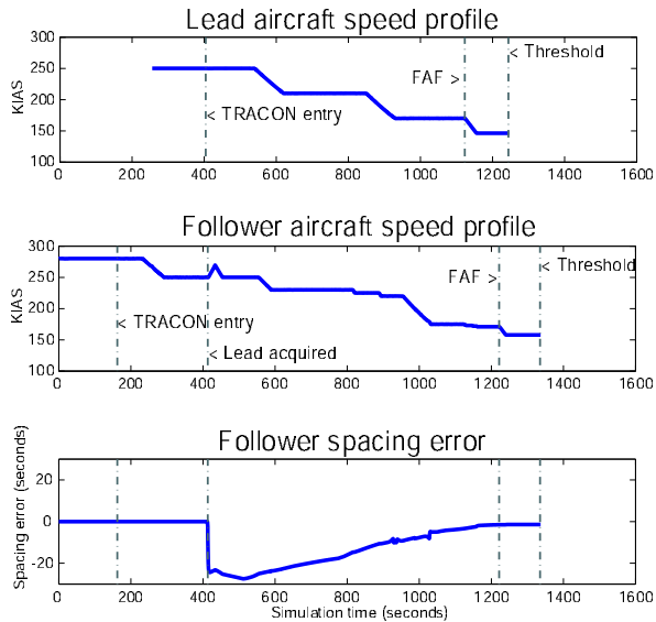
Fig. 3 Sample results of AMSTAR fast-time simulations with no winds. The top block shows the lead aircraft's current indicated airspeed while in profile mode. The middle block shows the trailing aircraft's indicated airspeed. The trailing aircraft starts in profile mode until the lead aircraft is acquired, it then transitions to paired mode. The bottom block shows the current spacing errors as calculated by the trailing aircraft.
