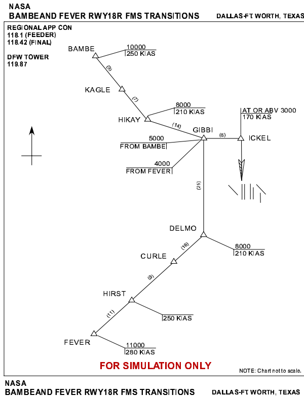
Fig. 2 Simulation approach routes for arrivals from the west landing at DFW runway 18R. Traffic merges laterally at GIBBI and vertically at ICKEL. Past ICKEL all aircraft intercept the 18R ILS.
