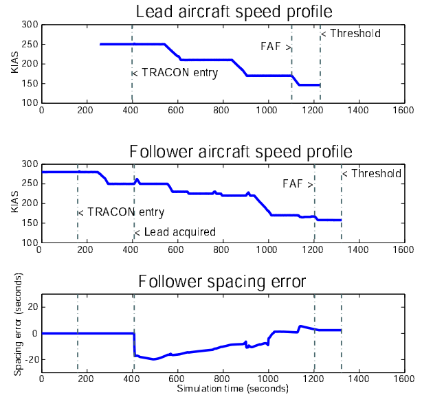
Fig. 4 Sample results of AMSTAR fast-time simulations with different truth and predicted wind fields. The top block shows the lead aircraft's current indicated airspeed while in profile mode. The middle block shows the trailing aircraft's indicated airspeed. The trailing aircraft starts in profile mode until the lead aircraft is acquired, it then transitions to paired mode. The bottom block shows the current spacing errors as calculated by the trailing aircraft.
