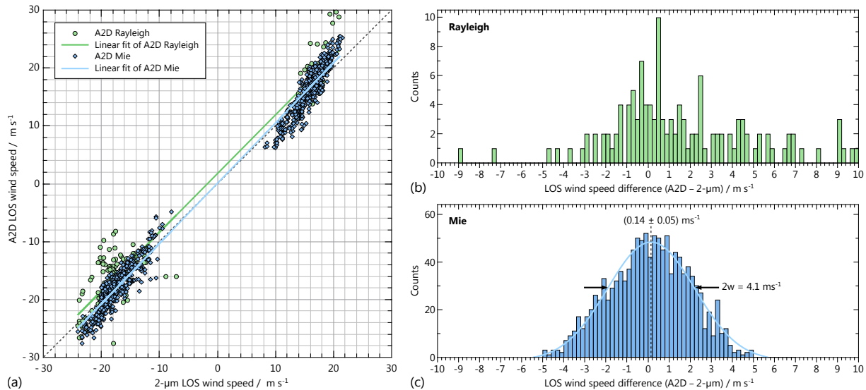
Figure 12. (a) A2D LOS wind speed determined with the Rayleigh (dots) and Mie (diamonds) channel versus the 2\ \mu\text{m} LOS wind speed for comparison of the wind data measured during the flight on 4 October 2016 between 09:00 and 10:30 UTC (see corresponding curtains in Fig. 11a, b and d). The scatterplot for the Mie channel was obtained after zero wind correction was applied to the measured wind speeds. The corresponding probability density functions for the wind differences (A2D– 2\ \mu\text{m} ) are shown in panels (b) and (c) for the Rayleigh and Mie channel, respectively. The solid line represents a Gaussian fit with the given centre and e^{-1/2} width 2w .
