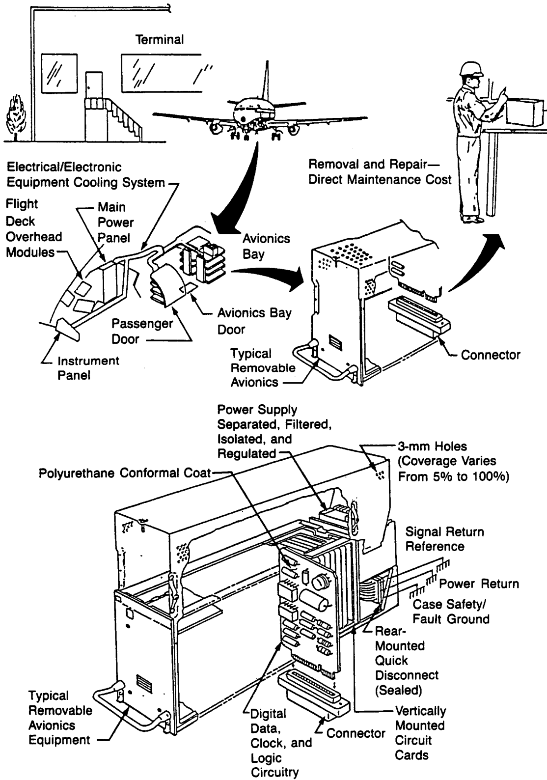
Figure 2.1-17 Line Replaceable Unit
