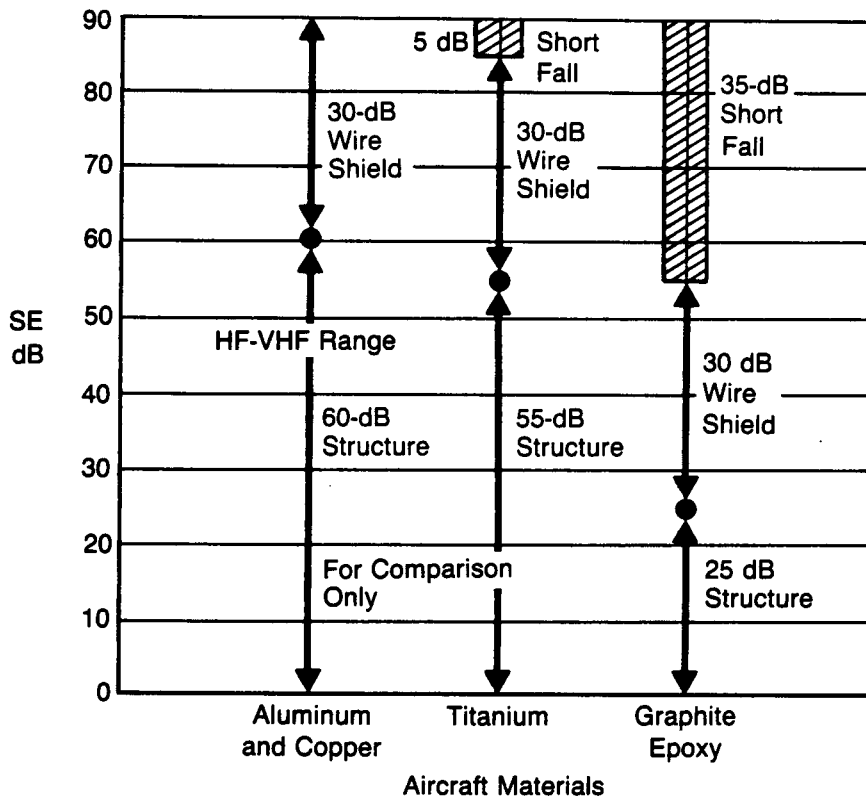
Figure 3.6-3 Graphite-Epoxy SE Shortfall
