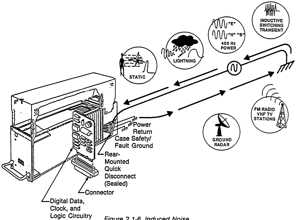
Figure 2.1-6 Induced Noise
