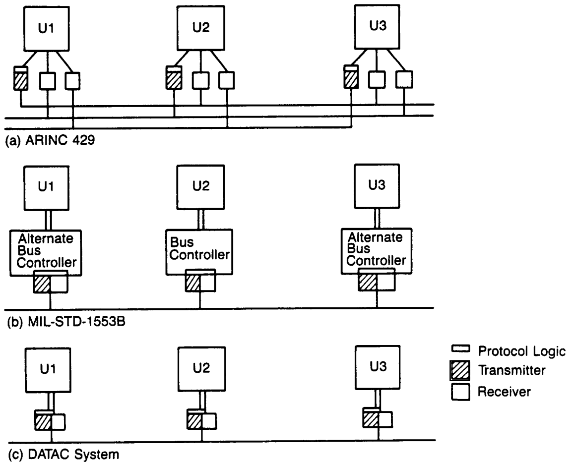
Figure 2.2-6 Digital Data Buses
