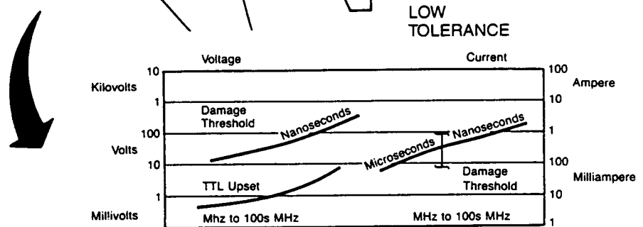
Figure 4.3-3 Trade—Digital Circuits
