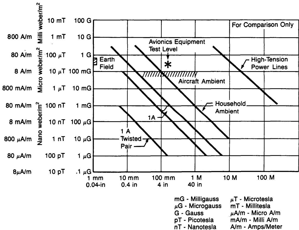
Figure 4.1-12 Magnetic Fields
