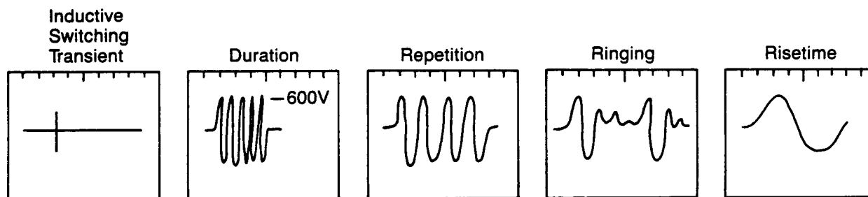
Figure 4.1-13 Transient Ringing
