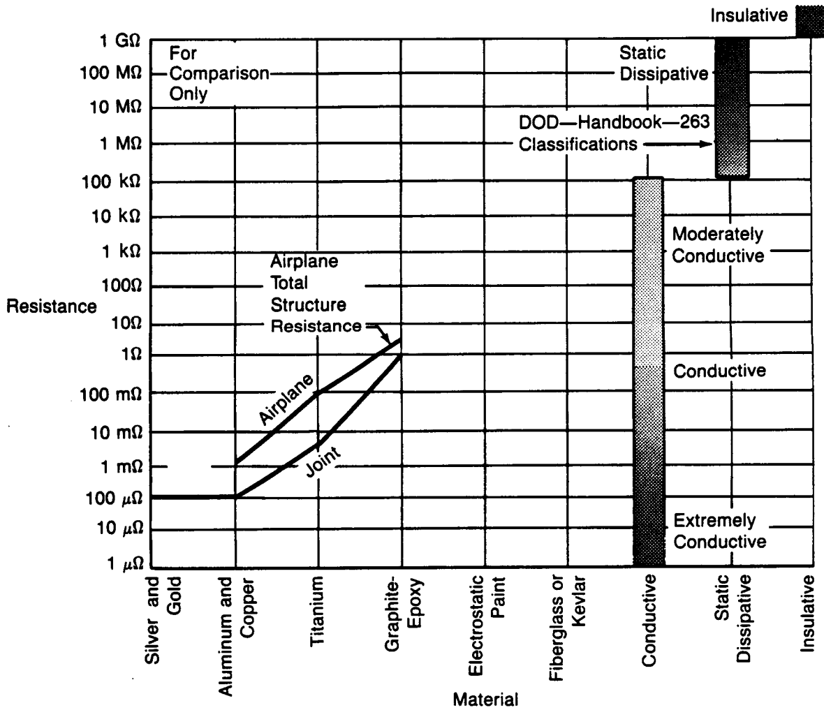
Figure 3.5-13 Configuration/Resistance Overview
