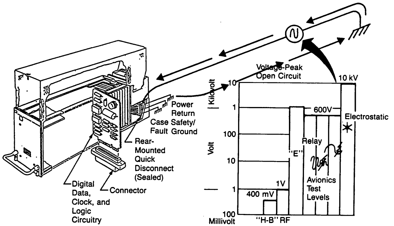
Figure 2.1-7 Noise Voltages
