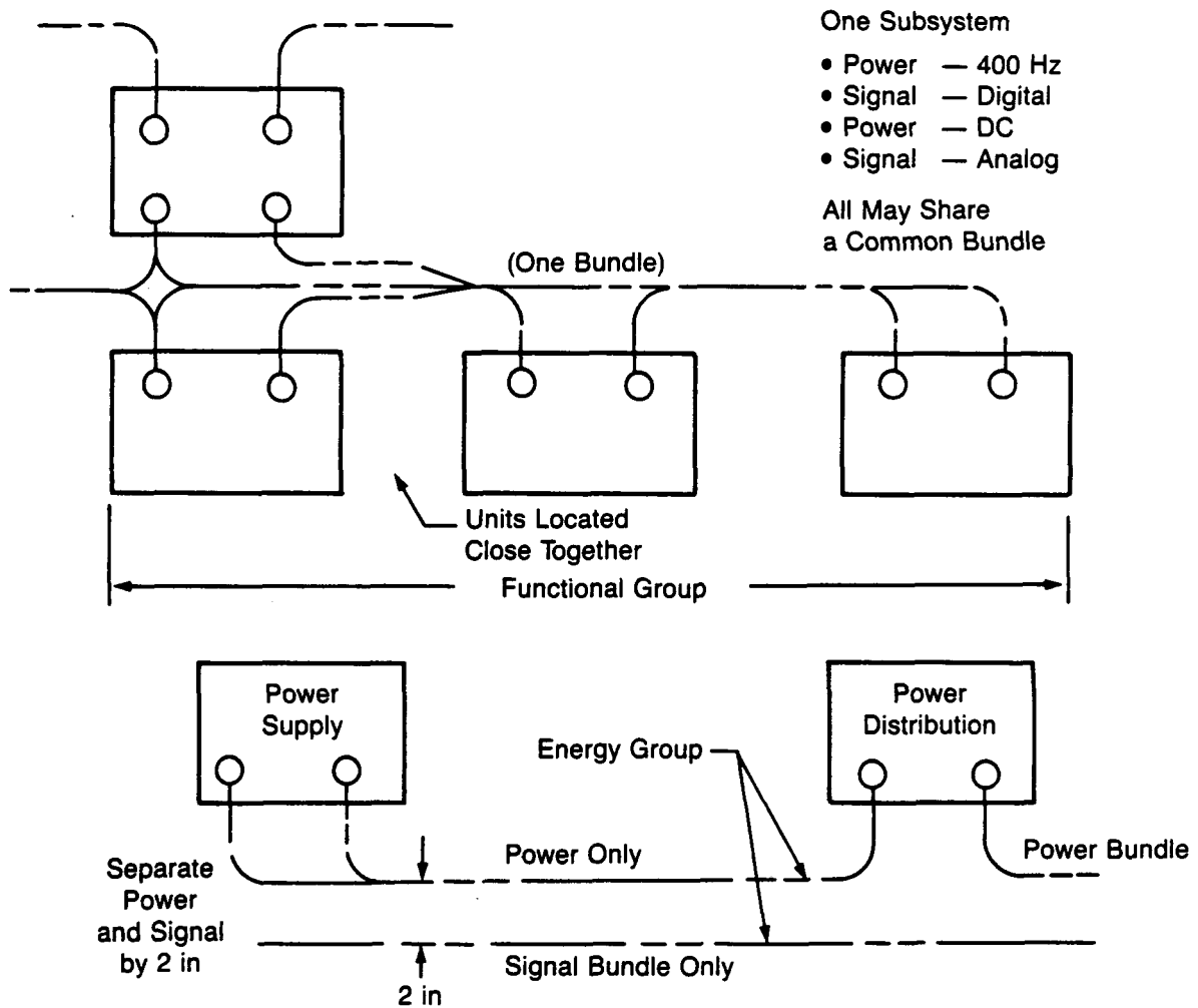
Figure 3.4-2 Wiring Categories
