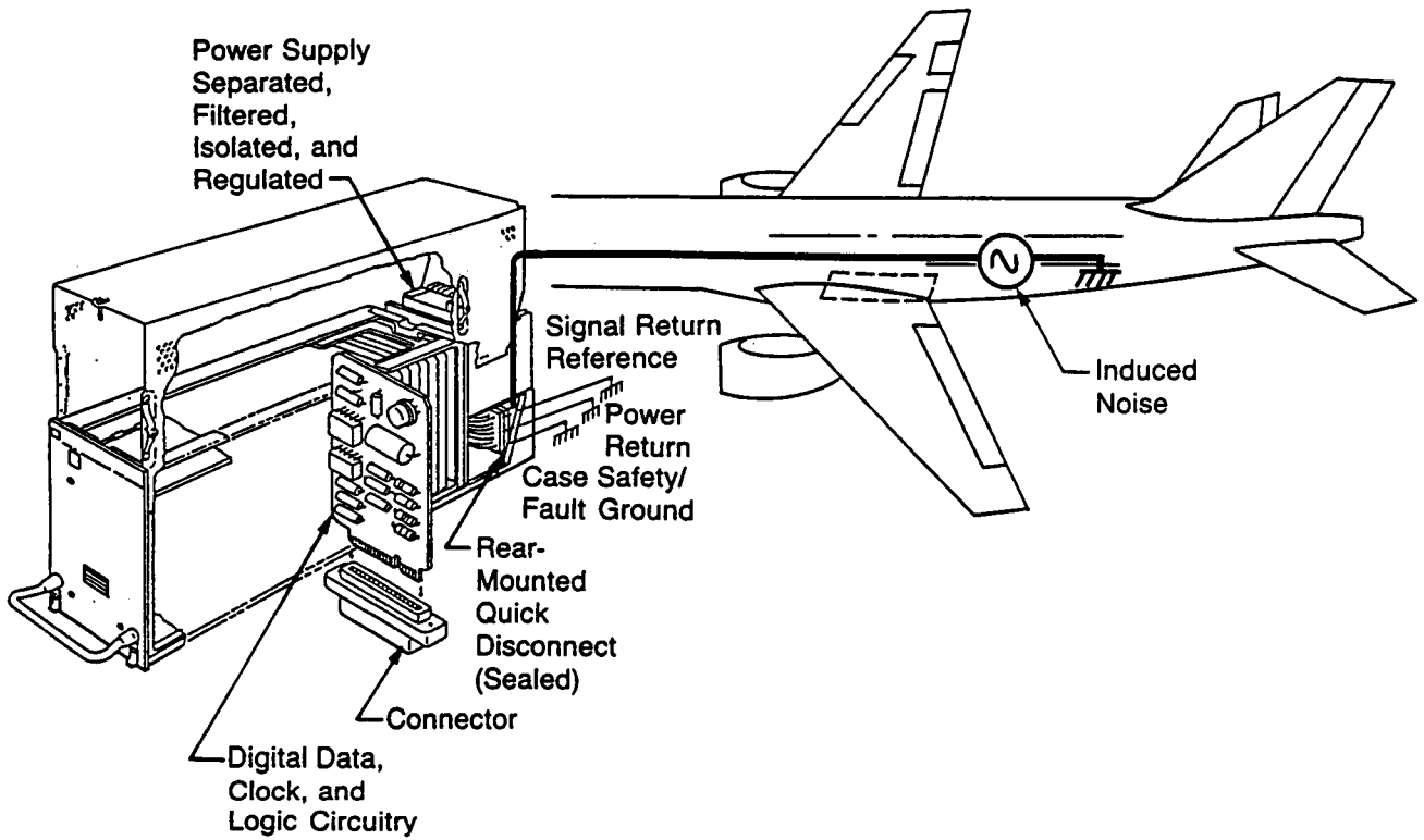
Figure 2.1-5 Structure Return
