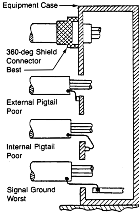
Figure 3.4-6 Shield Ties
