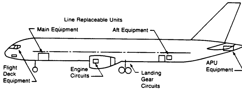
Figure 2.1-2 Avionics Bays
