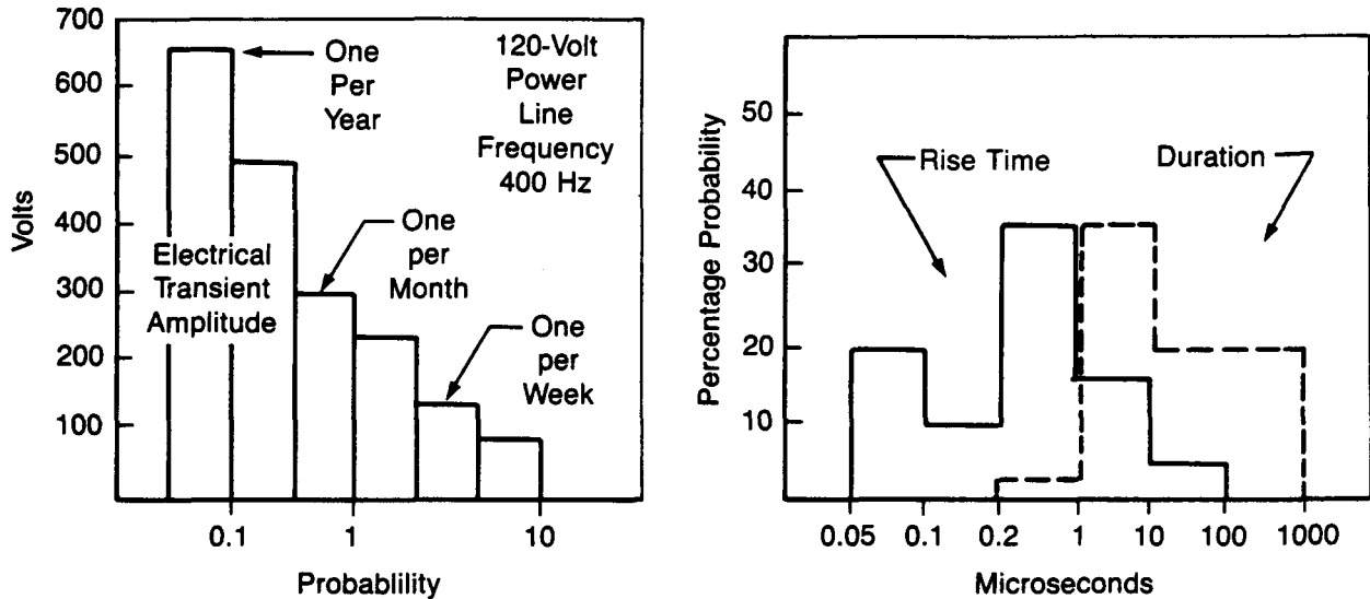
Figure 4.1-14 Electrical Transients
