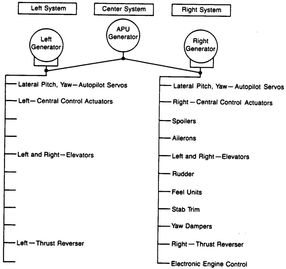
Figure 2.1-9 Separation Example
