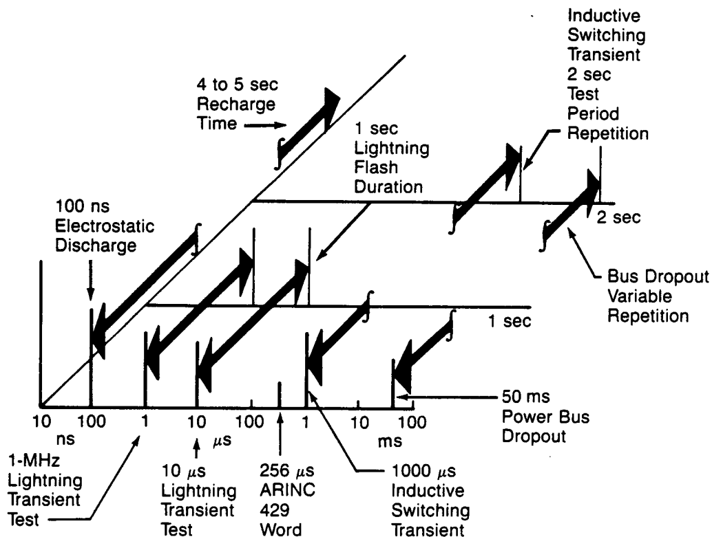
Figure 3.2-1. Transient Events
