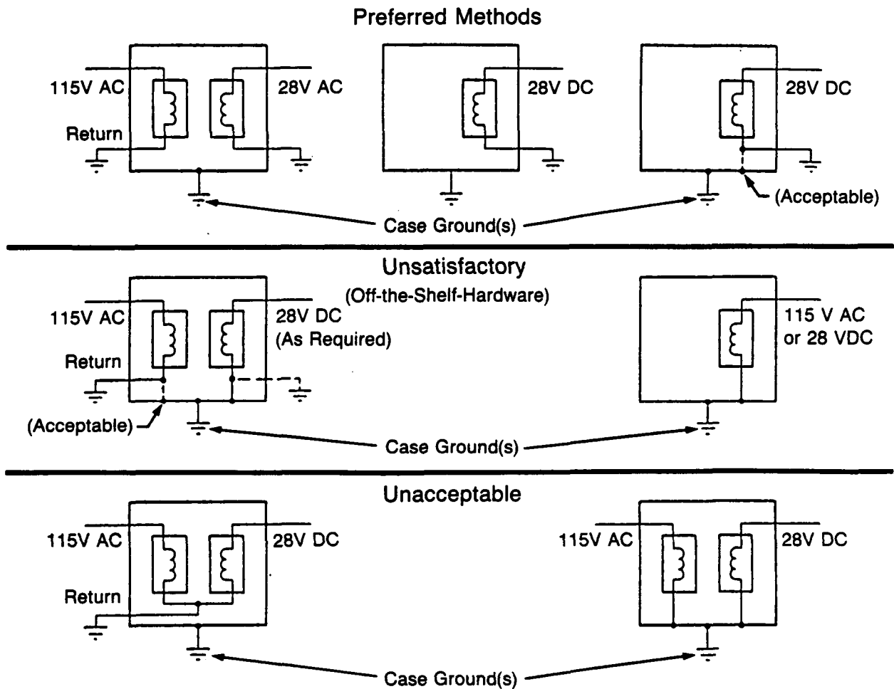
Figure 3.5-11 Power Returns
