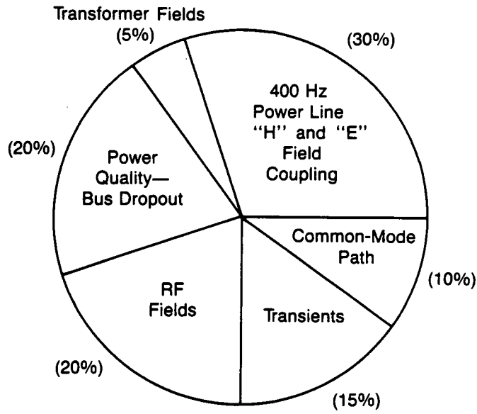
Figure 1.1-3 Percent Troubleshooting—A/C
