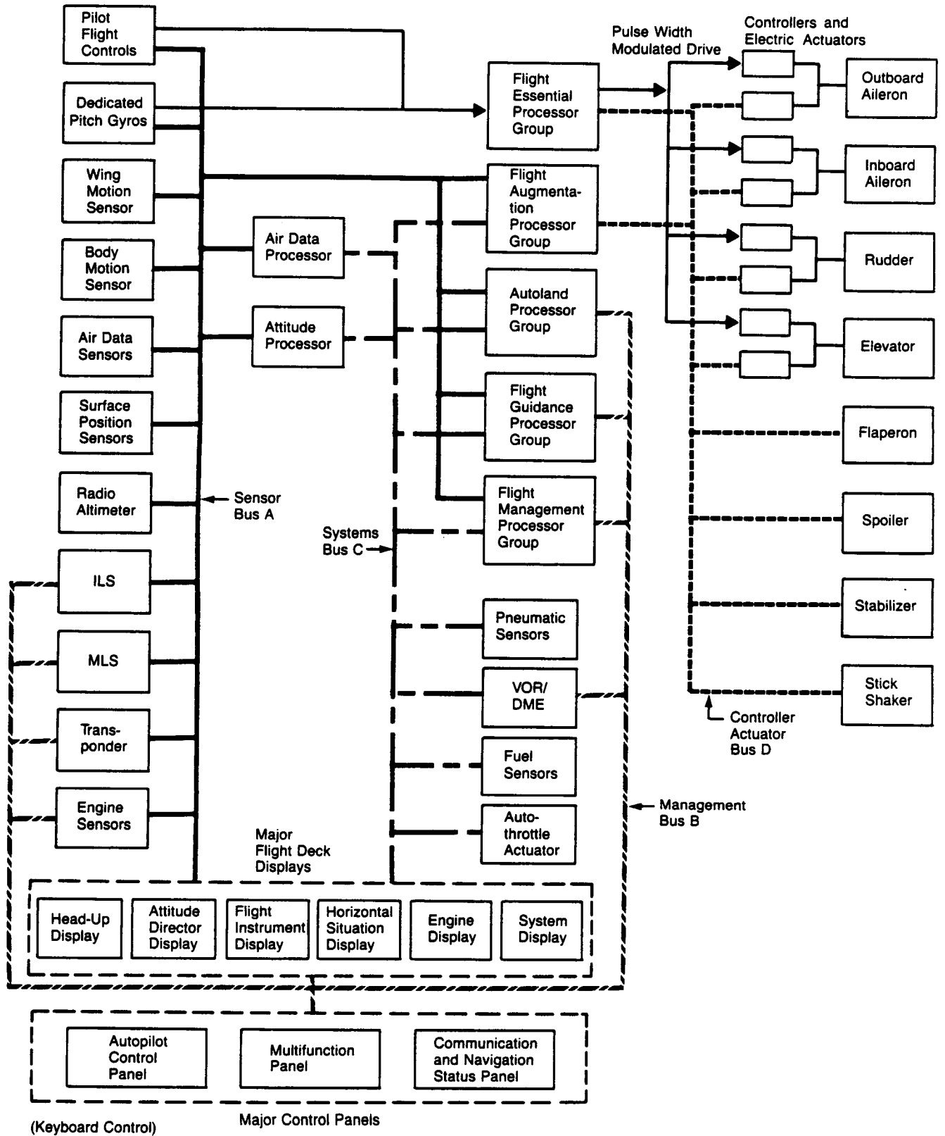
Figure 2.2-4 Hypothetical Architecture
