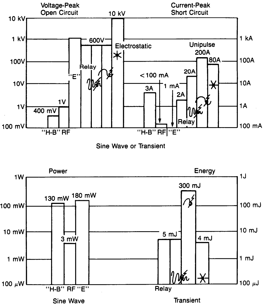
Figure 3.4-4 Selected EMI Levels
