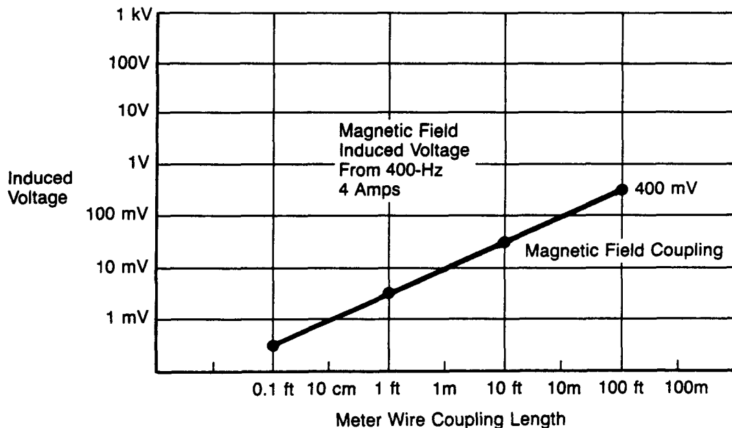
Figure 4.1-9 "H" Field Coupling
