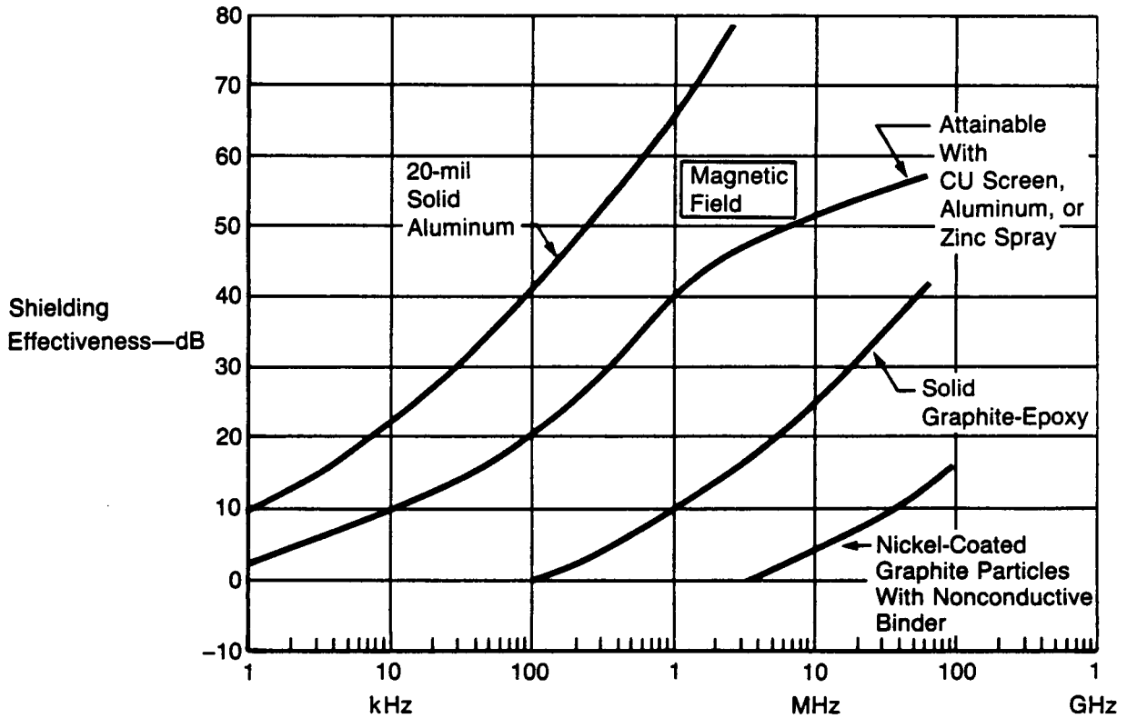
Figure 3.5-8 SE Comparison
