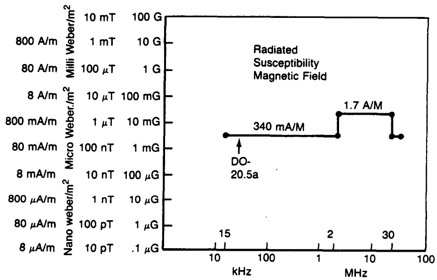
Figure B1. EMI Test Limits (Continued)
