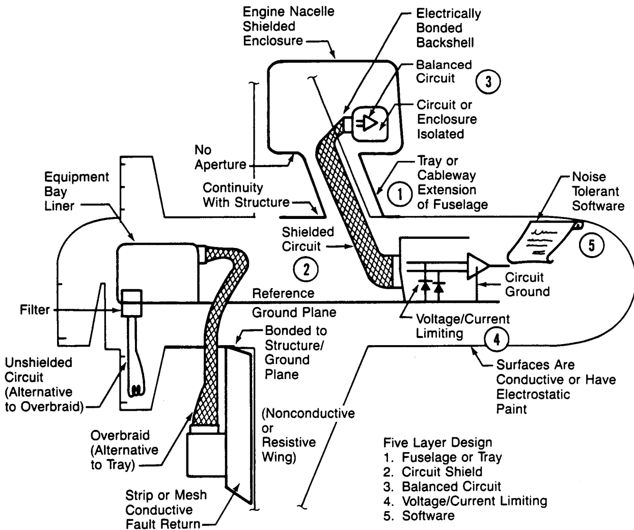
Figure 4.2-1 Layered Design
