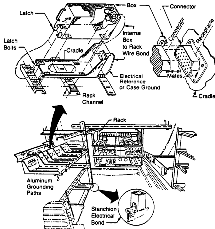
Figure 2.1-4 Main Bay Aluminum Structure
