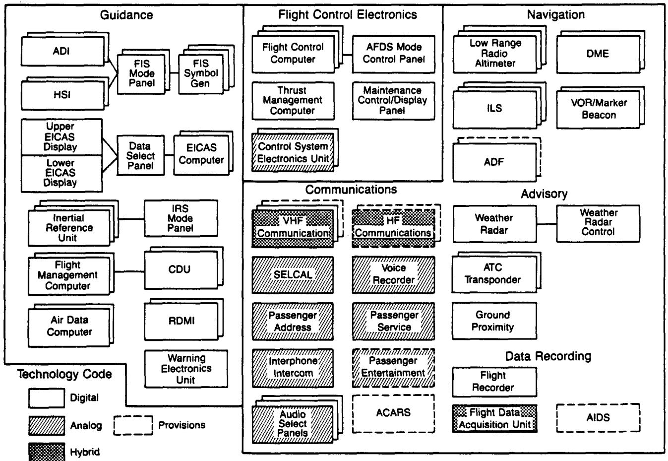
Figure 2.1-18 Flight Management Systems
