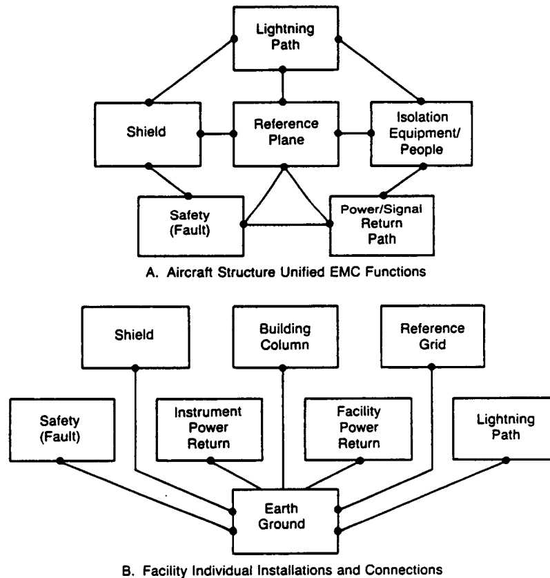
Figure 3.5-5 EMC Anatomy Block Diagram
