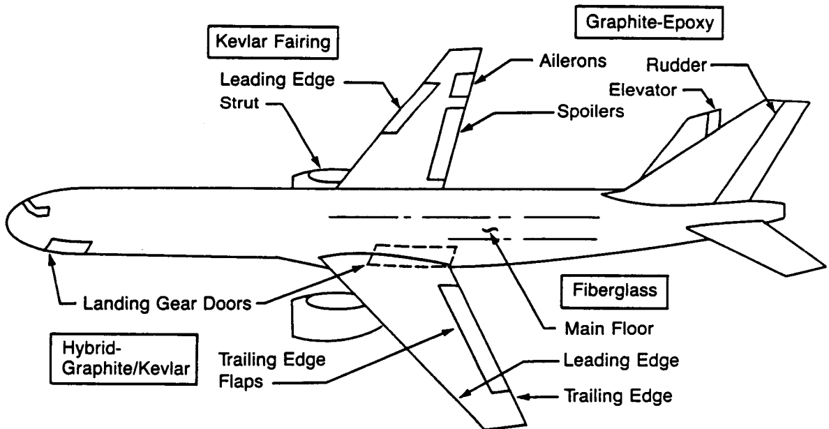
Figure 2.1-8 Nonmetallic Interfaces
