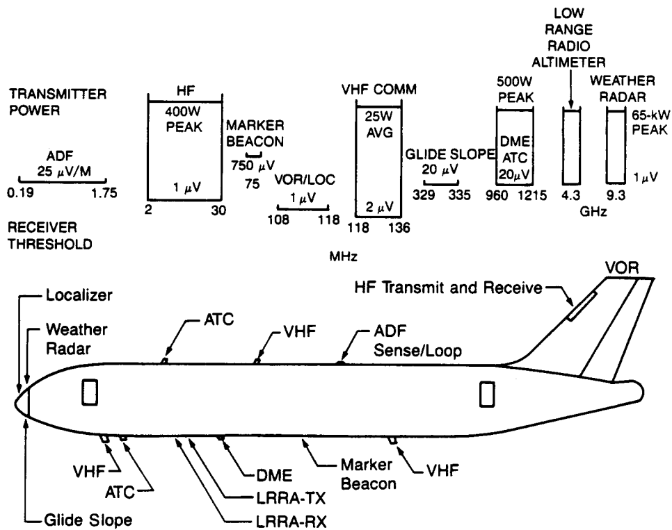
Figure 2.1-12 Transmitters-Receivers
