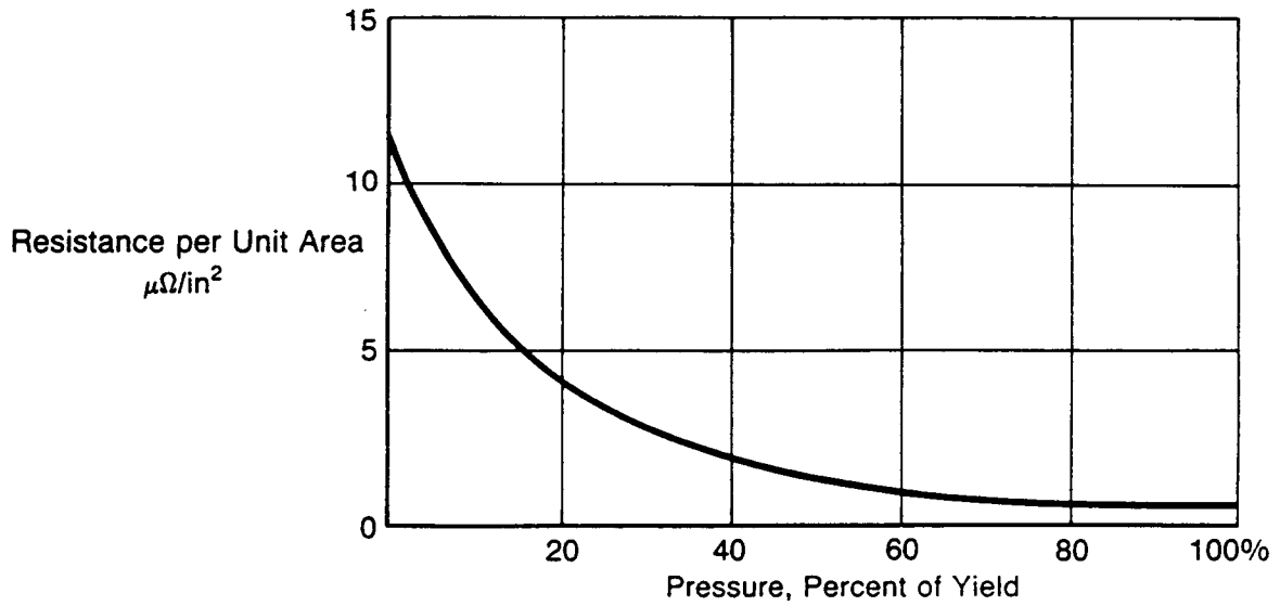
Sections of 2024 Aluminum Alloy Under Compression With Joint Sanded Prior to Test
