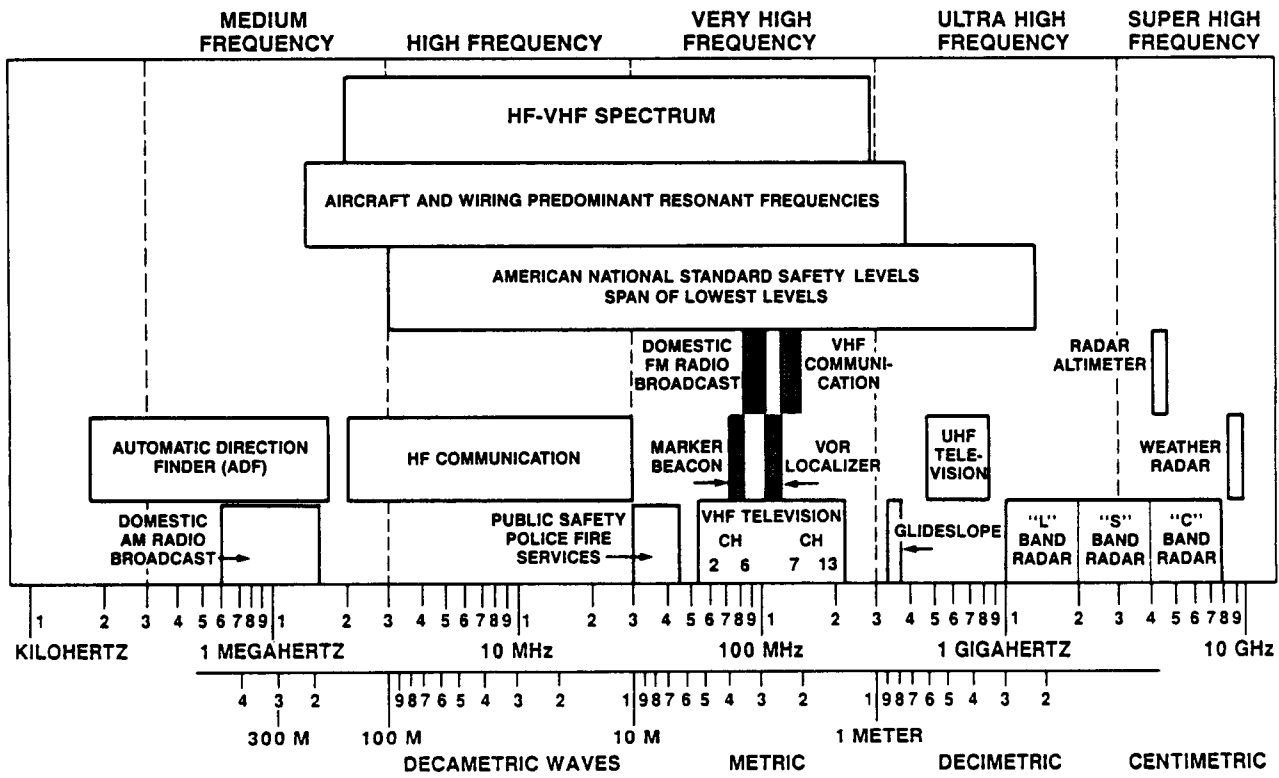
Figure 4.1-1 HF-VHF Range
