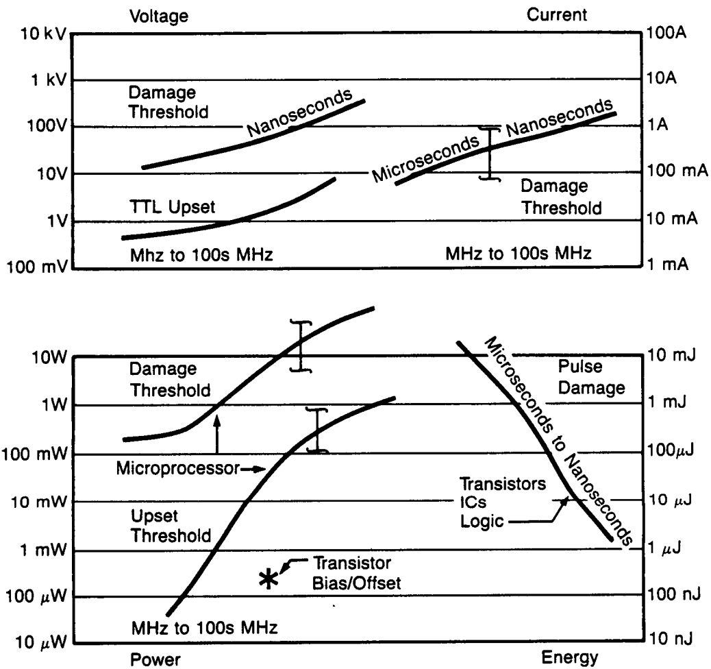
Figure 3.1-1 Microcircuit Tolerance
