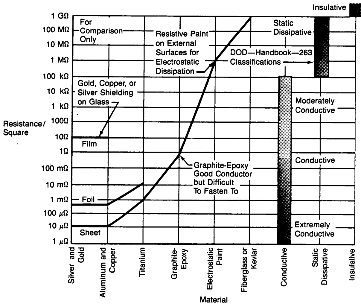
Figure 3.5-12 Material/Resistance Overview
