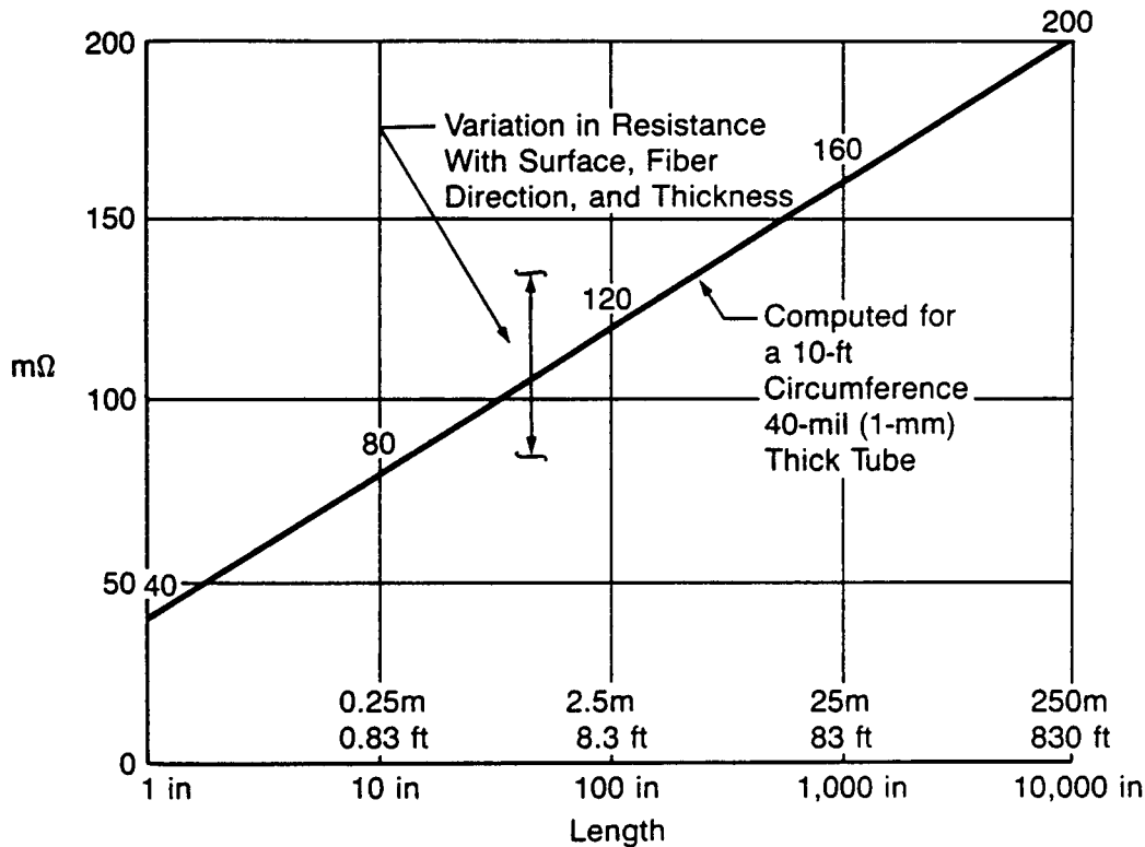
Figure 3.6-2 Graphite-Epoxy Resistance
