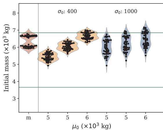
Fig. 14. Prior test in relation with the true mass data. Green horizontal lines refer to m_{oew} and m_{mtov} . \sigma_0 grouped by different colors. (For interpretation of the references to colour in this figure legend, the reader is referred to the web version of this article.)
