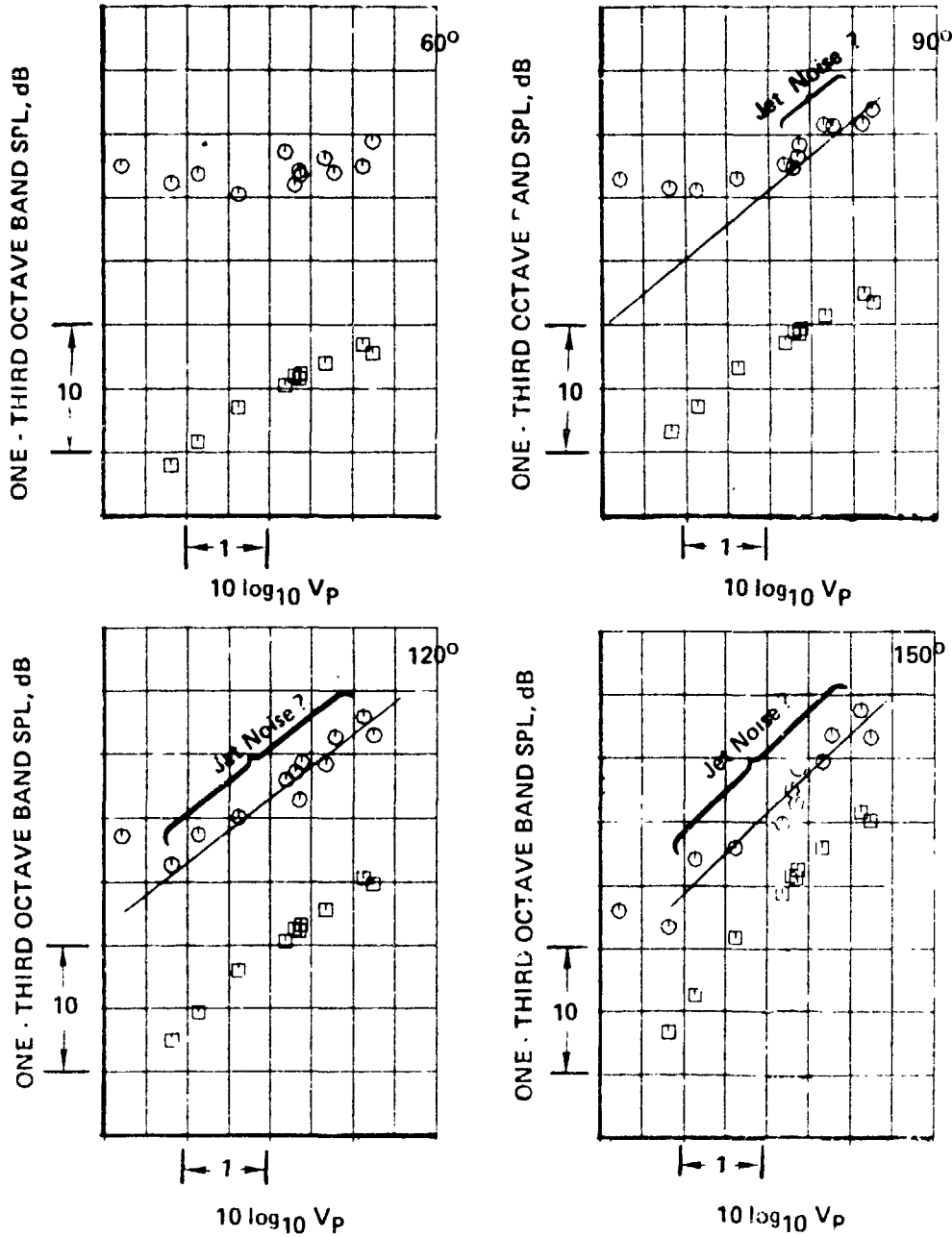
Figure 27.--SPL Comparisons as a Function of Primary Jet Velocity
