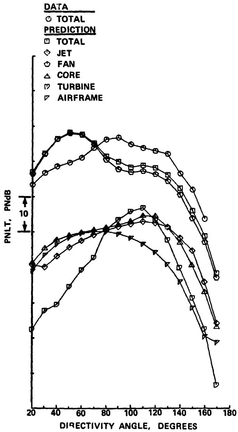
(e) ENGINE POWER SETTING, % N1C = 91.0
