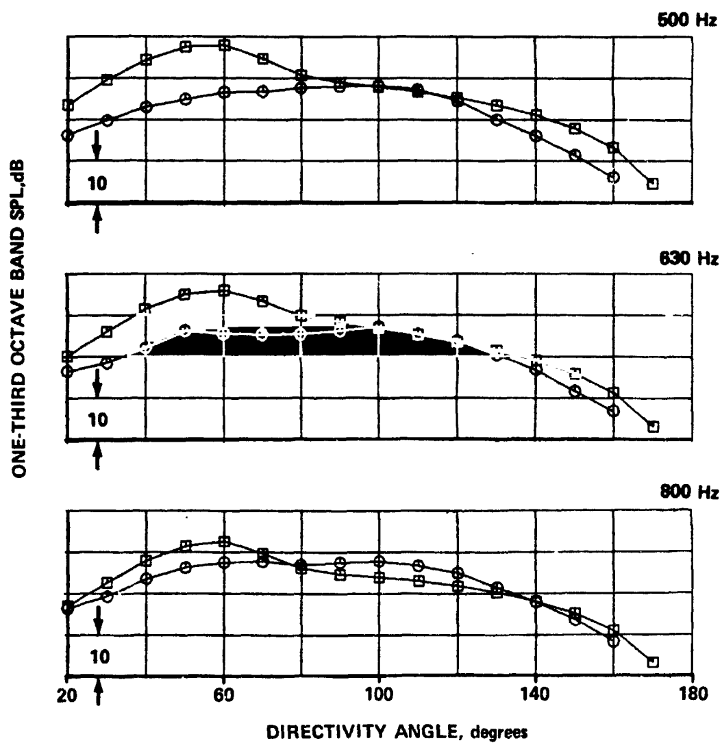
b) TAKEOFF POWER 500-800Hz
