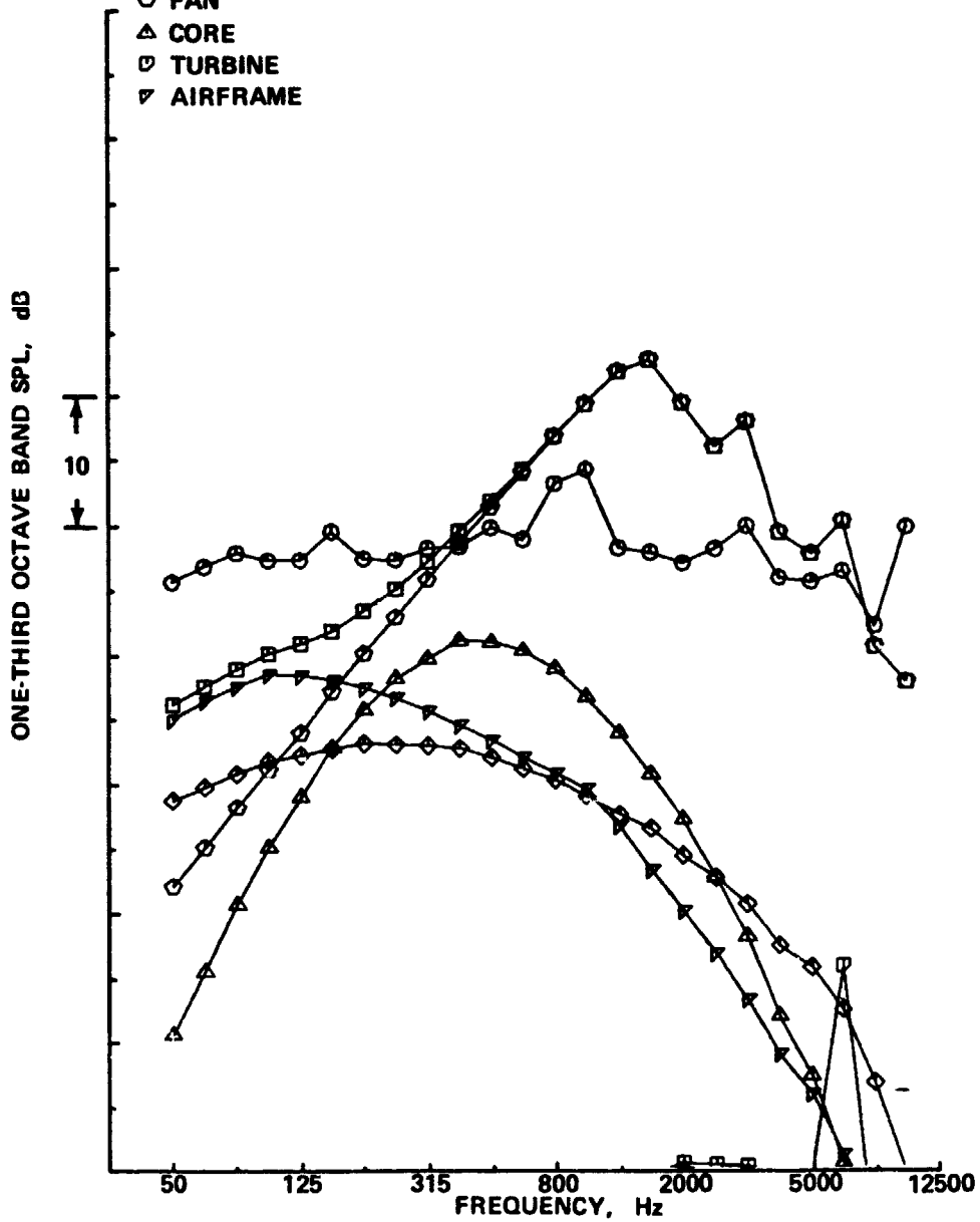
Figure A5. — Spectral Comparisons of Data and Prediction, Engine Power Setting % N 1C = 90.7
