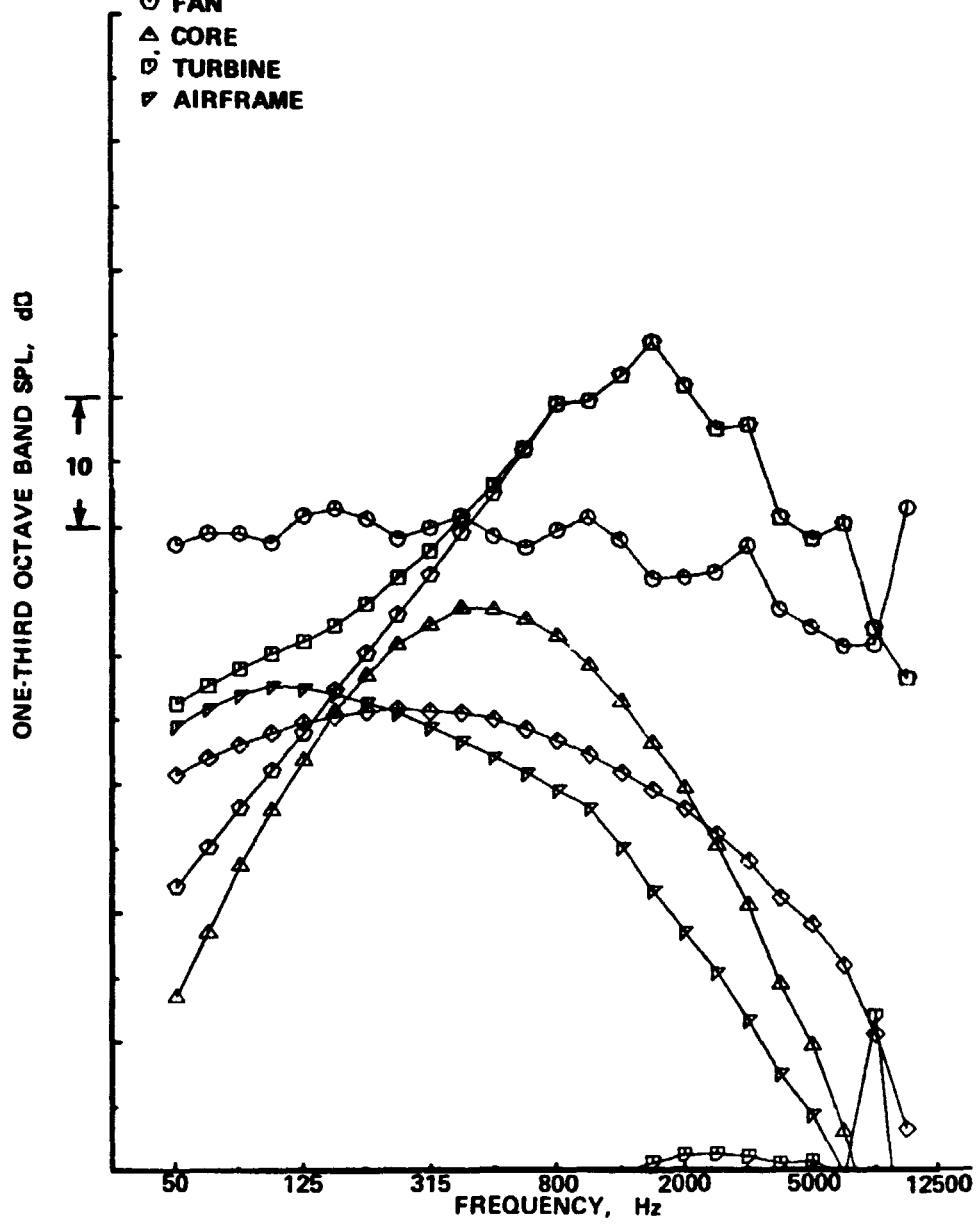
Figure 12. — Spectral Comparisons of Data and Prediction at Takeoff Power
