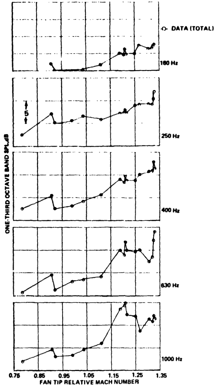
(a) DIRECTIVITY ANGLE 30°
