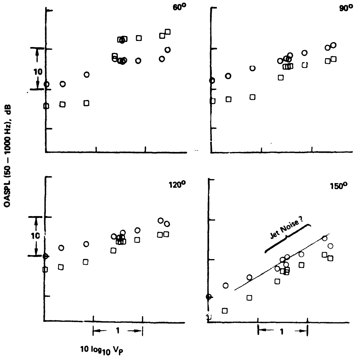
Figure 26. - Overall SPL Comparisons as a Function of Primary Jet Velocity
