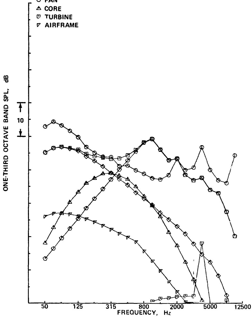
(e) DIRECTIVITY ANGLE = 150°
