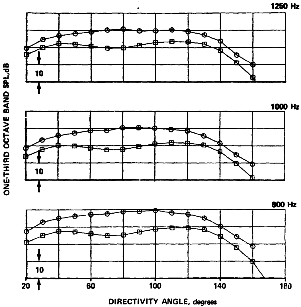
e) APPROACH POWER 800-1250 Hz
