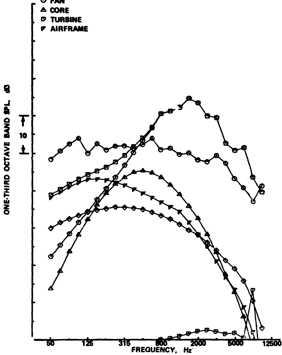
Figure A1. — Spectral Comparisons of Data and Prediction, Engine Power Setting % N 1C = 98.8
