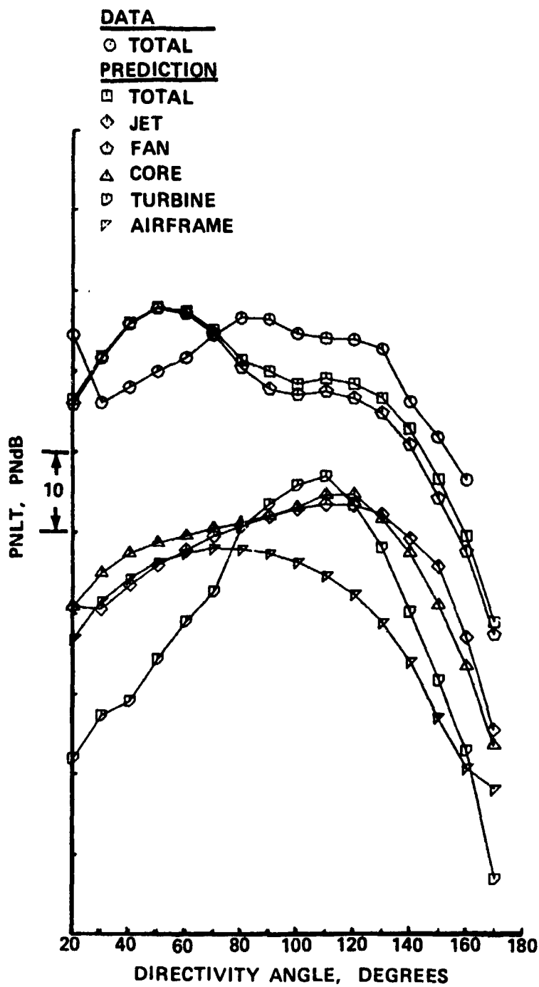
(f) ENGINE POWER SETTING, % N1C = 91.3
