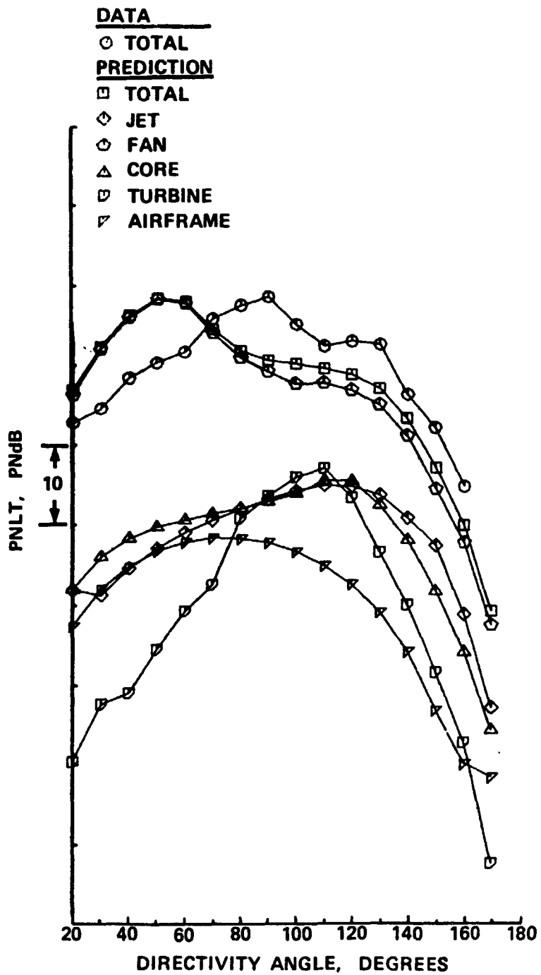
(c) ENGINE POWER SETTING, % N1C = 93.7
