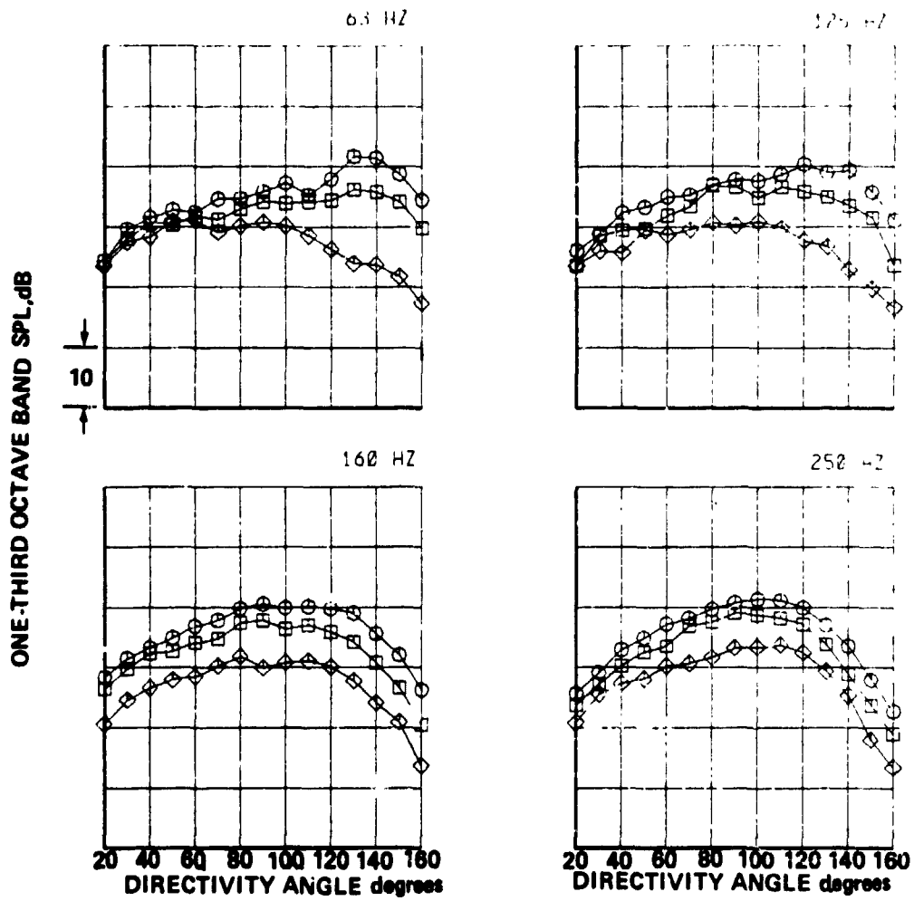
(a) FREQUENCY 63 TO 250 Hz
