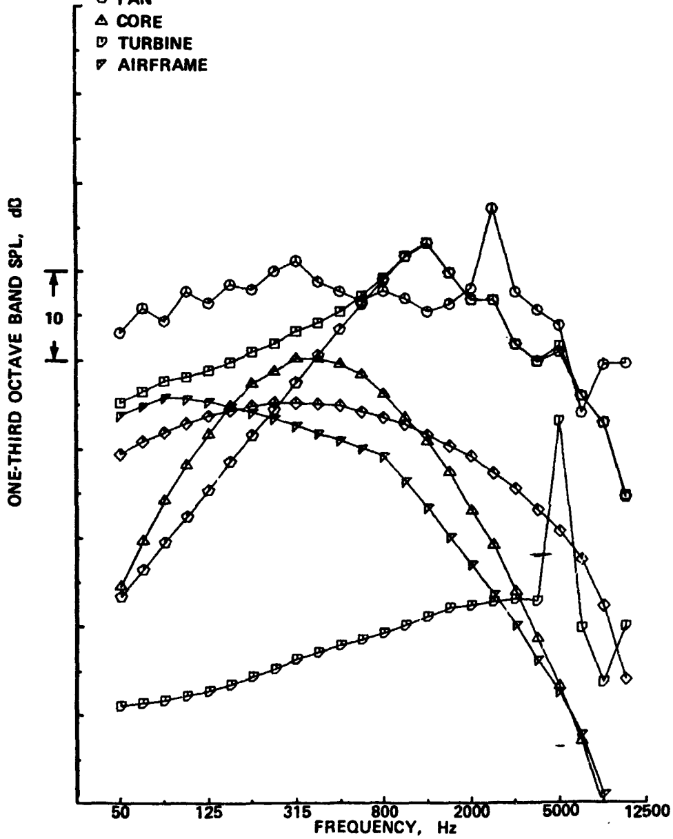
(c) DIRECTIVITY ANGLE = 90°
