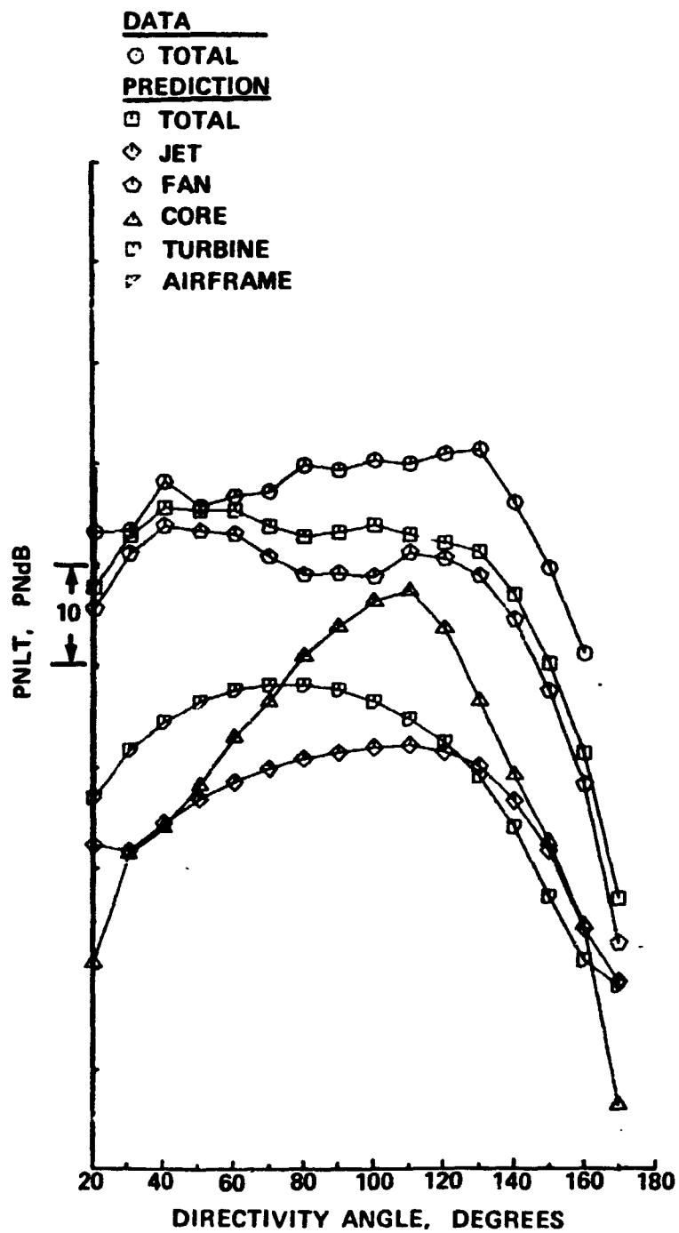
(j) ENGINE POWER SETTING, % N1C = 75.4
