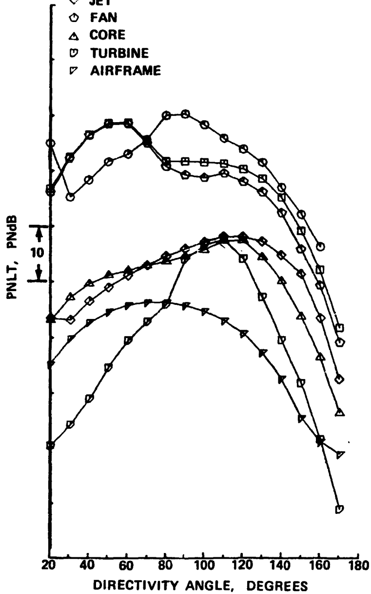
(b) ENGINE POWER SETTING, % N1C = 98.2
