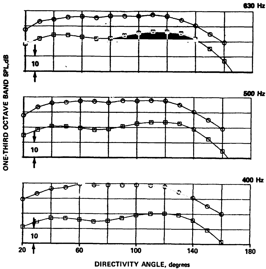
f) APPROACH POWER 400-630 Hz
