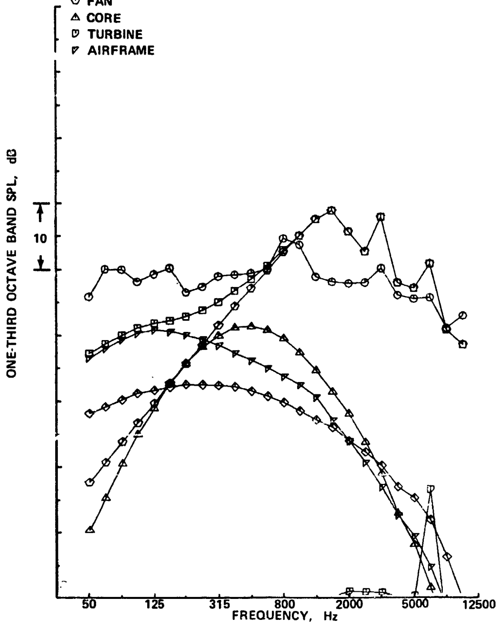
Figure A3. - Spectral Comparisons of Data and Prediction, Engine Power Setting % N 1C = 89.5
