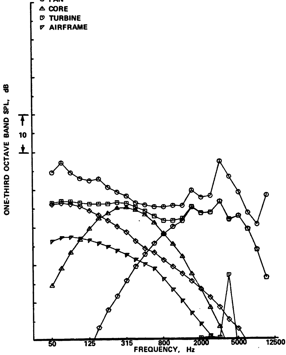
(e) DIRECTIVITY ANGLE = 150°
