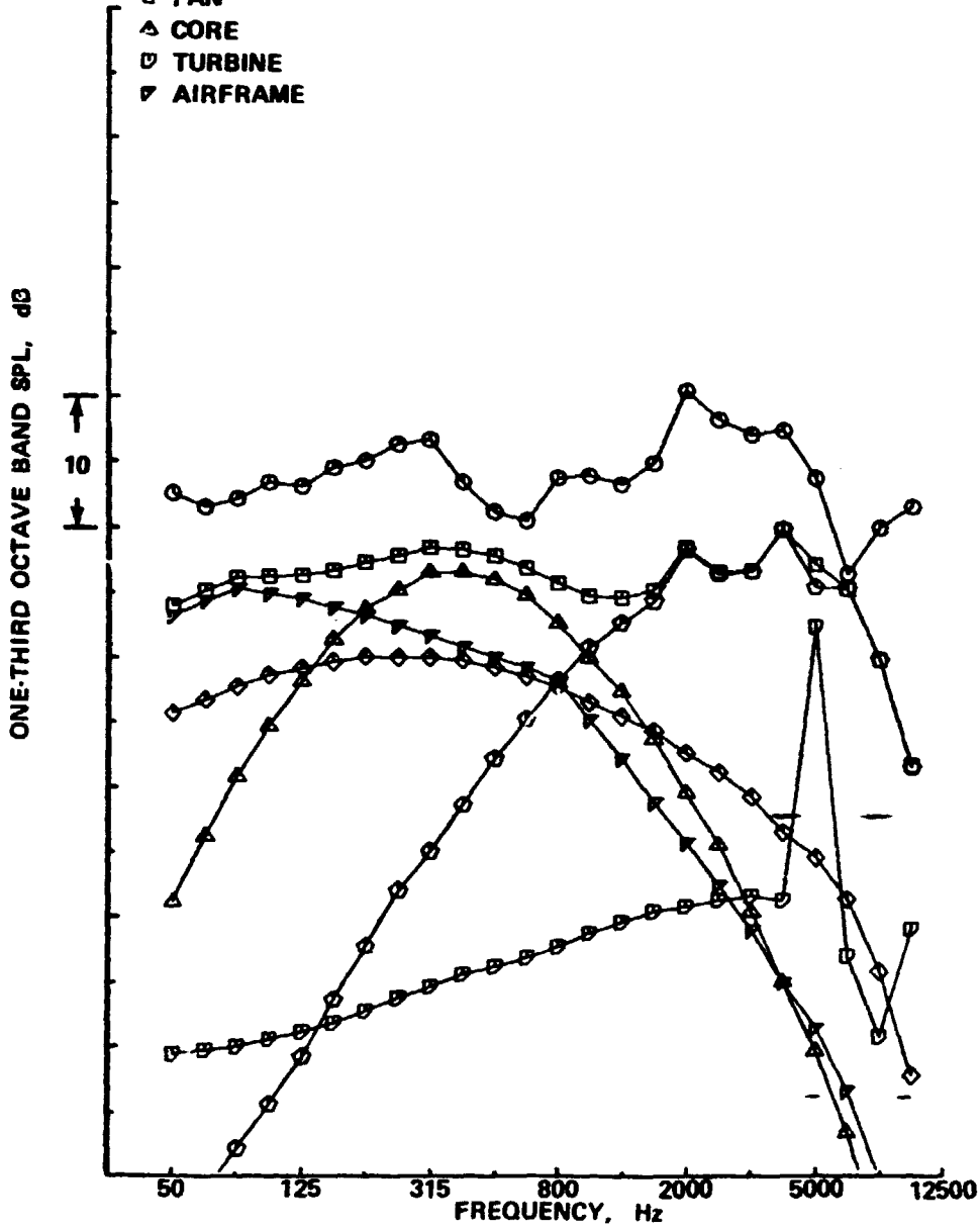
(c) DIRECTIVITY ANGLE = 90°
