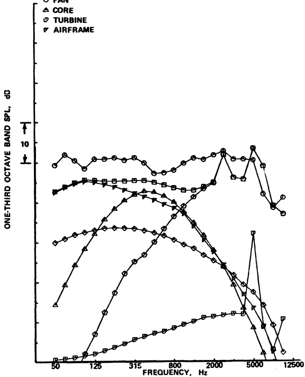
(b) DIRECTIVITY ANGLE = 60°
