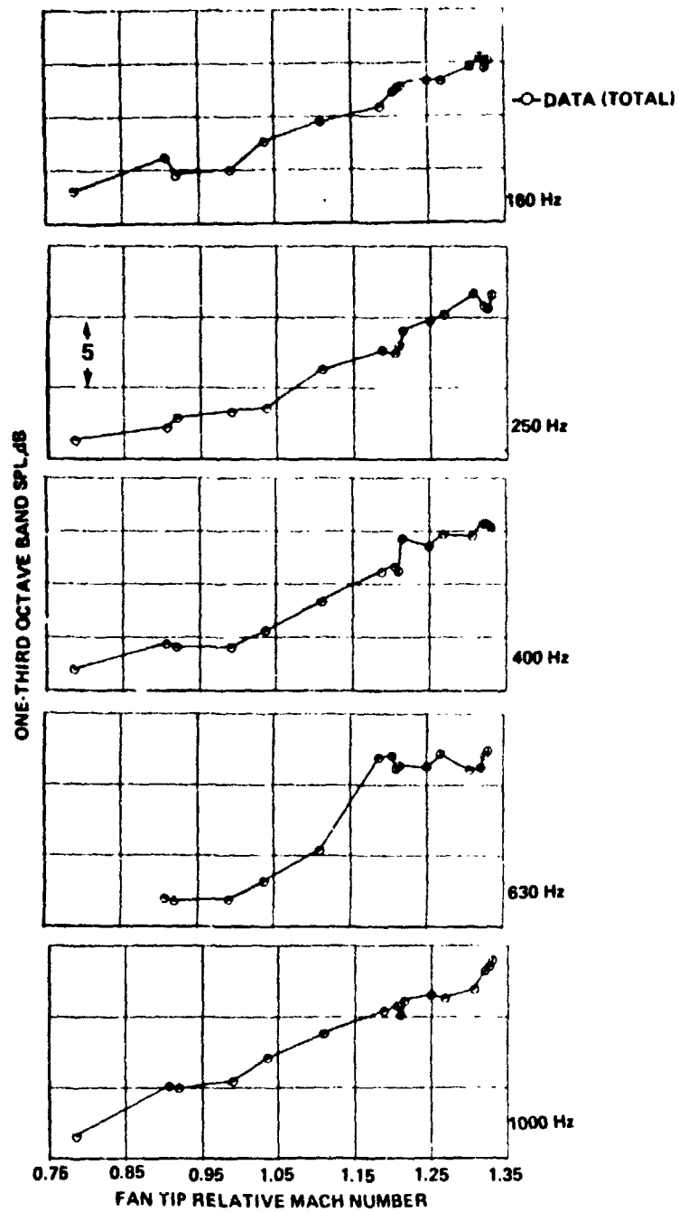
(c) DIRECTIVITY ANGLE 90°
