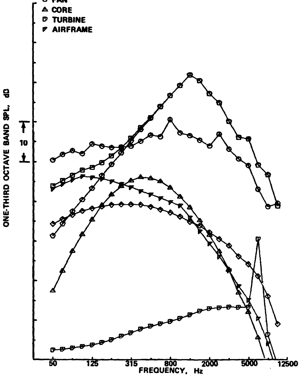
(b) DIRECTIVITY ANGLE = 60°
