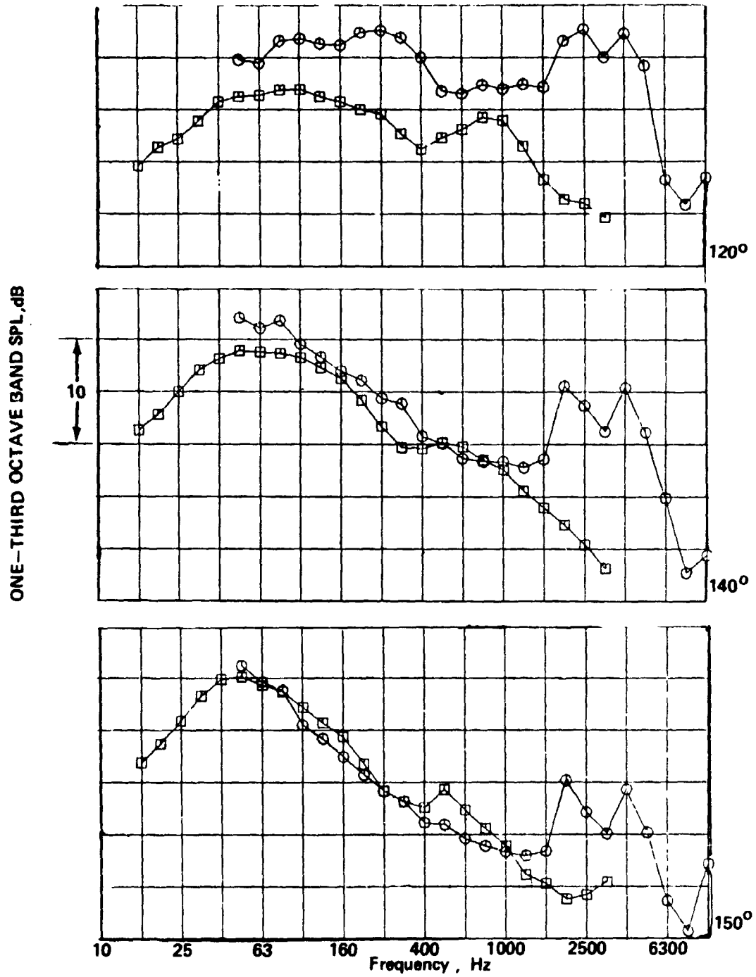
Figure 24. --Spectral Comparisons of 747/JT9D Flyover and Model Scale Jet Noise Data
