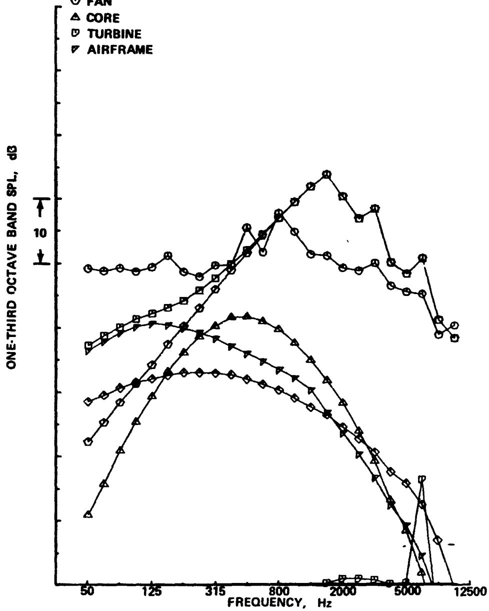
Figure A4. — Spectral Comparisons of Data and Prediction, Engine Power Setting % N 1C = 91.0
