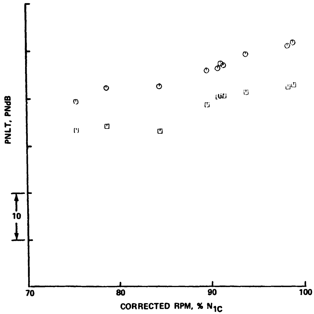
c) Directivity Angle 90°
