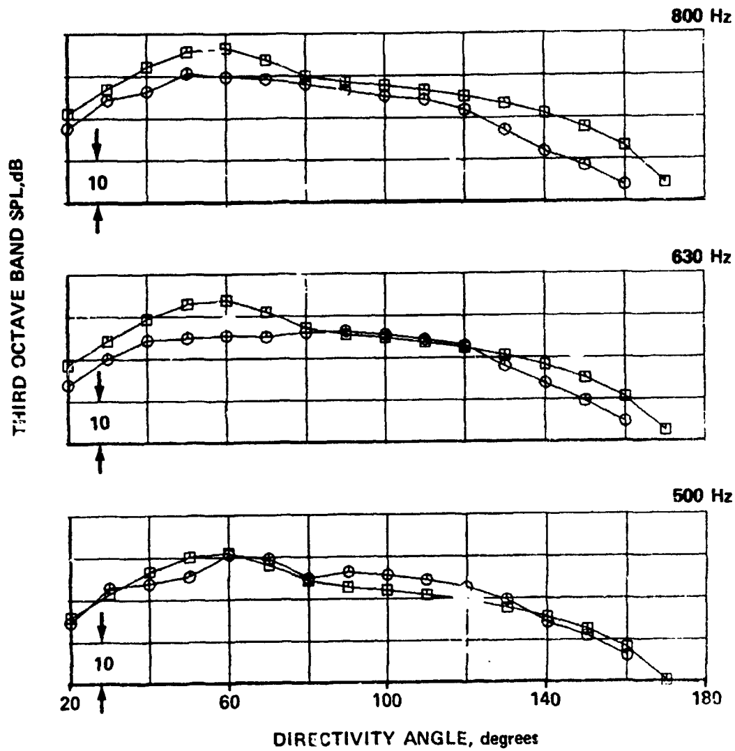
d) CUTBACK POWER 500-800 Hz
