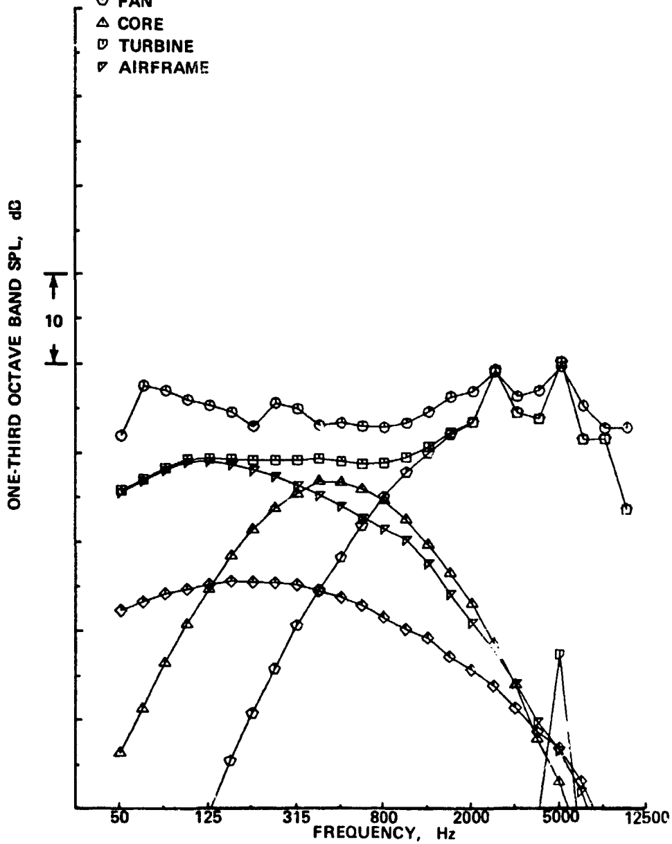
(a) DIRECTIVITY ANGLE = 30°
