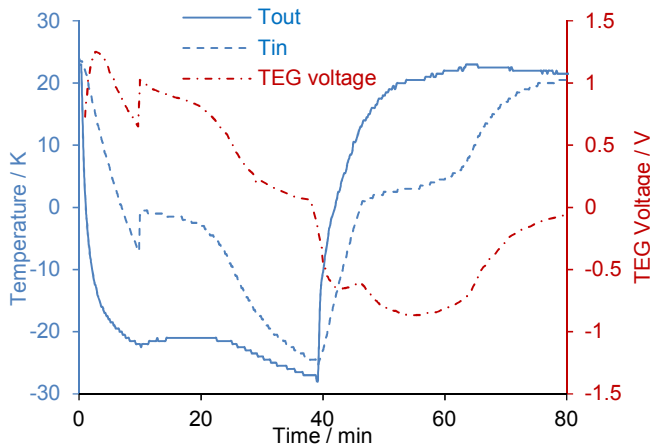
Fig. 10: Harvester temperature and voltage response to a temperature cycle corresponding to a typical flight.
