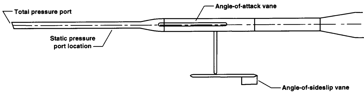
Figure 2. Noseboom for measuring pitot and flow angles.
