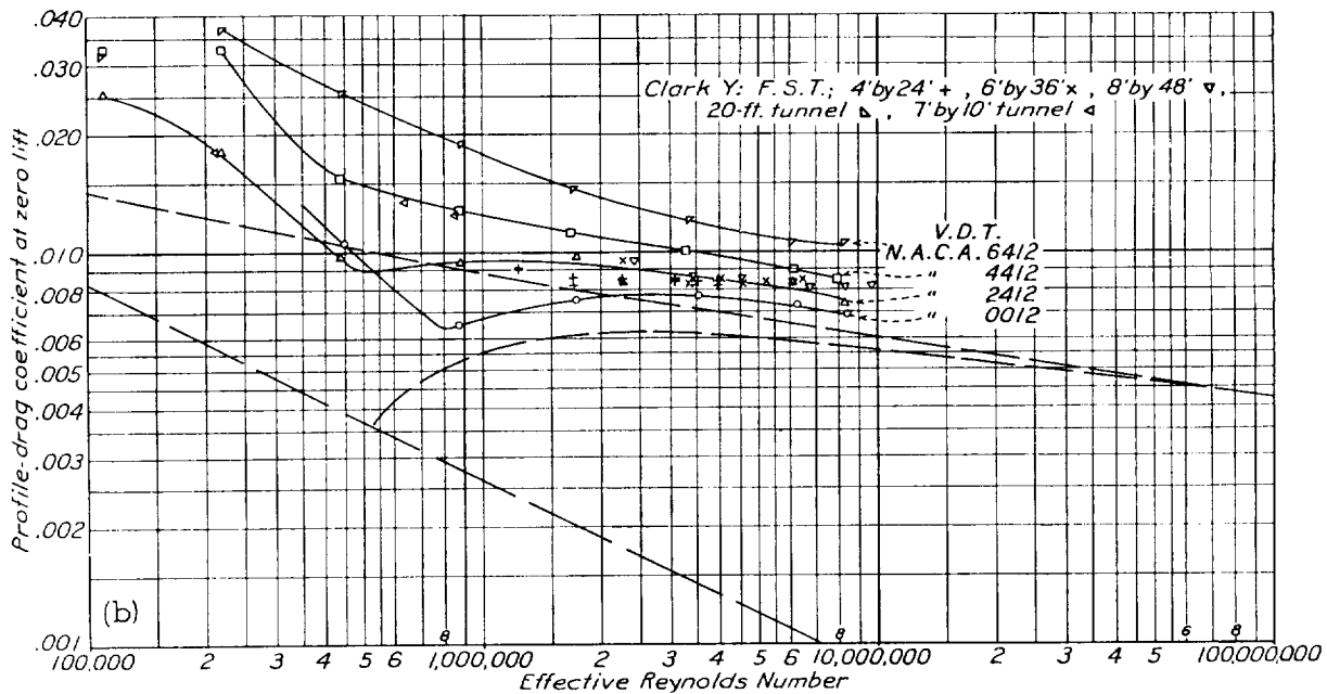
FIGURE 41.—Profile-drag coefficient.
