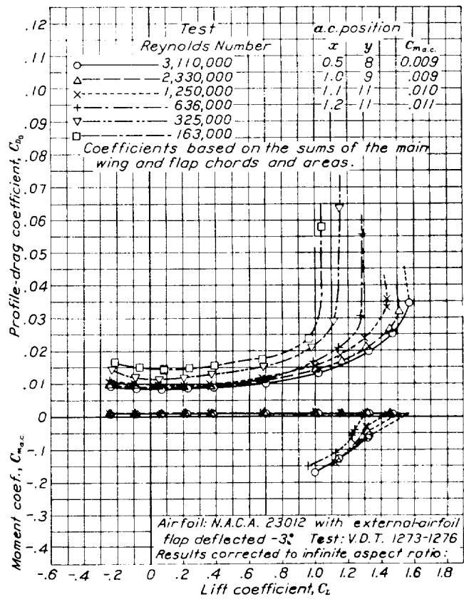
FIGURE 22.—N. A. C. A. 23012 with external-airfoil flap deflected -3°.
