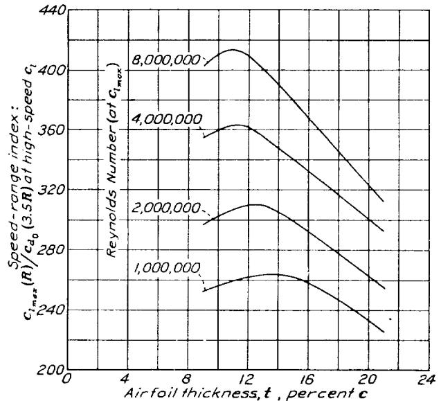
FIGURE 25.—Airfoil speed-range indexes for various Reynolds Numbers. N. A. C. A. 230 series sections; c_{l,max} taken for airfoil with 0.20c split flap deflected 75°; c_{d0} taken for airfoil with flap retracted for a high-speed value of c_l and at 3.5 times the R for the c_{l,max} .
