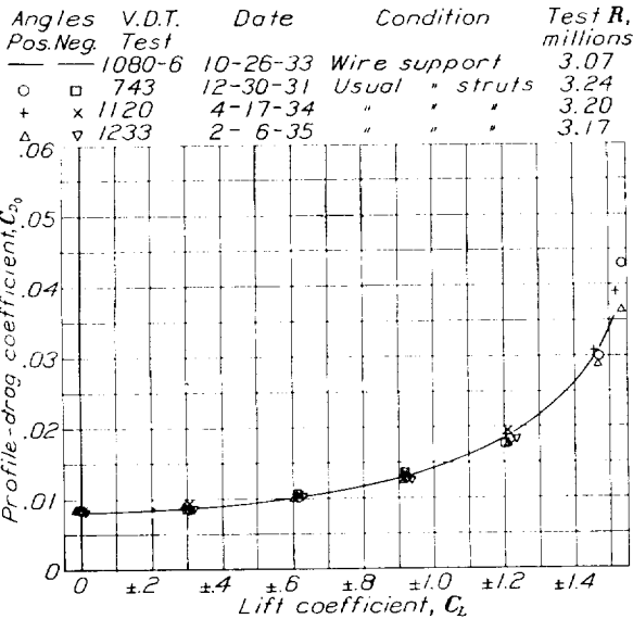
FIGURE 46.—Lift and drag characteristics of the N. A. C. A. 0012 airfoil as determined from tests with the model mounted on the usual support struts and on special wire supports.
