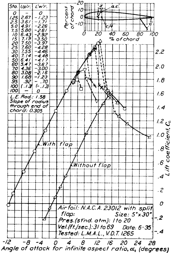
FIGURE 17.—N. A. C. A. 23012 with split flap deflected 60°.
