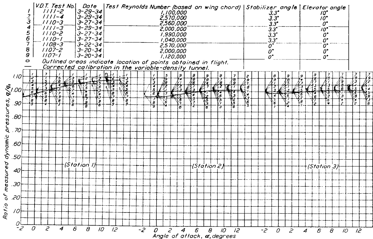
FIGURE 49.—Calibration of pitot tubes mounted on the FC-2W2 airplane in flight and on the FC-2W2 airplane model in the variable-density wind tunnel. Results corrected for tunnel-wall effect.
