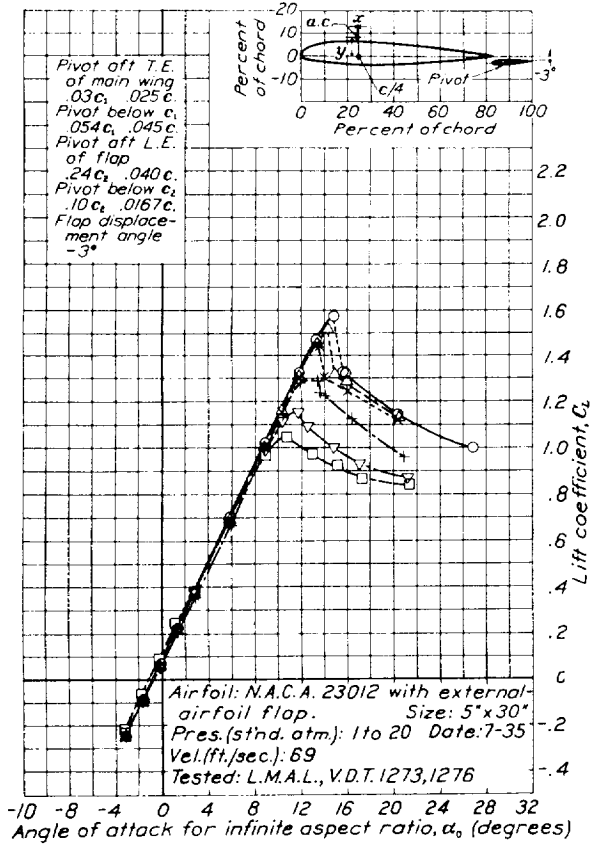
FIGURE 22.—N. A. C. A. 23012 with external-airfoil flap deflected -3°.
