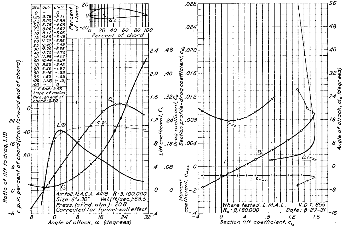
FIGURE 47.—N. A. C. A. 4418 airfoil.
