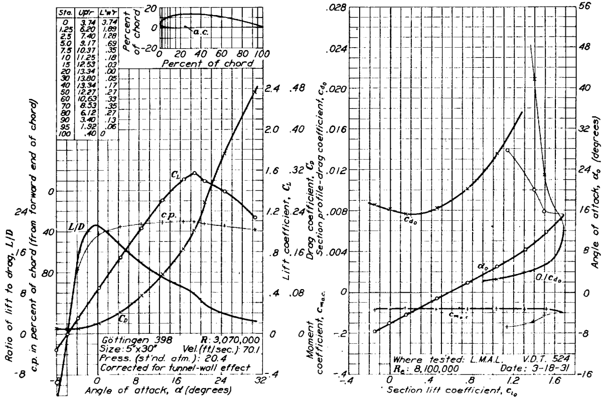
FIGURE 23.—Göttingen 398 airfoil.
