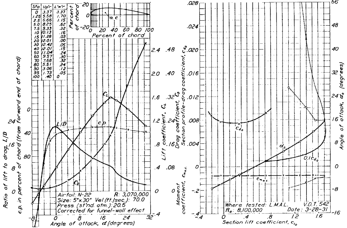
FIGURE 24.—N-22 airfoil.
