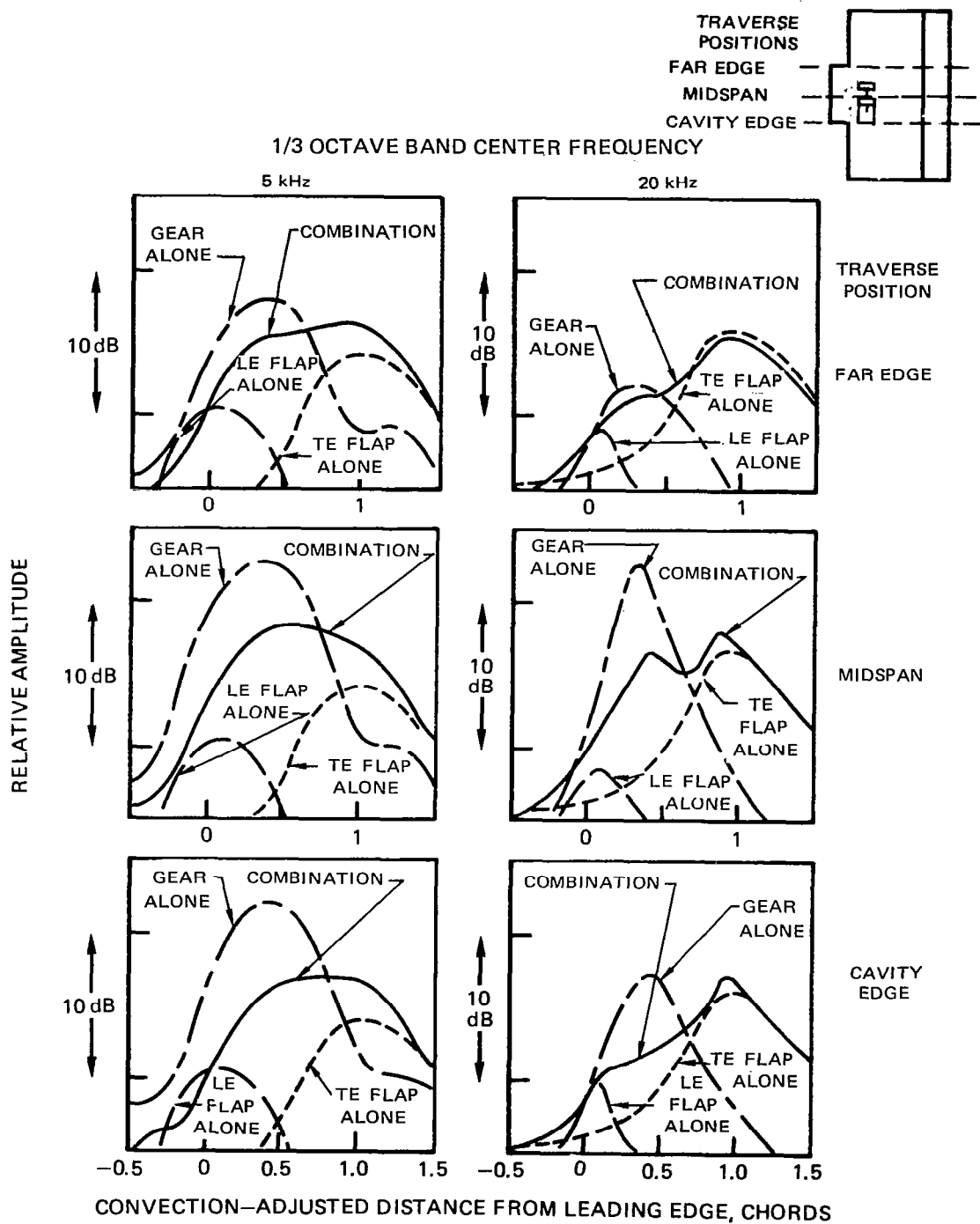
Figure 66 — Comparison of Noise Source Strength Distributions for Leading Edge Flap, Landing Gear Midspan, Full Span Trailing Edge Flap Combination with those of Components Alone
