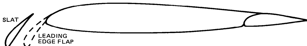
(d) WING AND 15% CHORD, 25^\circ DEFLECTION SLAT INSTALLED AS EITHER A LEADING EDGE FLAP OR LEADING EDGE SLAT
