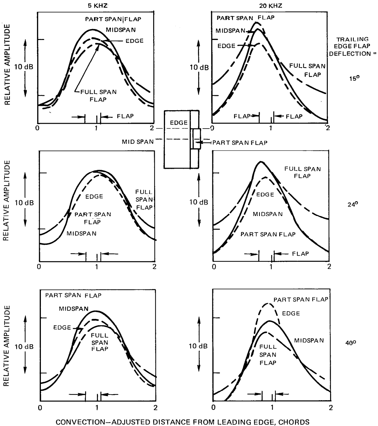
Figure 28 – Variation of Noise Source Strength Distribution with Spanwise Position on a Part-Span Single Slotted Trailing Edge Flap at 100 M/Sec Velocity
