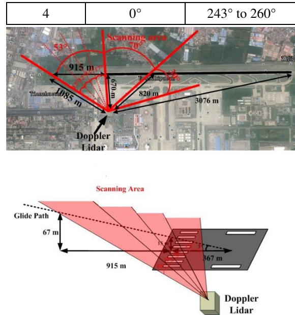
Figure 1 Location and scanning strategies of PCDL that configured at BCIA.
