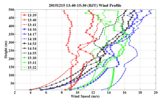
Figure 2 Wind speed profiles measured by PCDL at BCIA on Dec 15 th , 2015.
