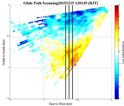
Figure 3 Glide path scanning of 36L/18R runway at BCIA on Dec 15 th , 2015.
