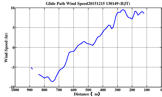
Figure 4 Wind speed profiles measured by PCDL at BCIA on Dec 15 th , 2015.
