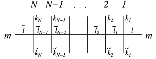
FIG. 2. Construction of the Monodromy matrix: the matrix element (\mathcal{T}_m)_{l, k_N \dots k_1}^{\bar{l}, \bar{k}_N \dots \bar{k}_1} is equal to the total Boltzmann weight of the m th row, for a fixed configuration of external arrows (specified by the indices of \mathcal{T}_m ), obtained by summing over all allowed configurations of arrows on internal lines (whose indices carry bars here).
