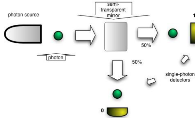
Fig. 1. Optical system for generating quantum random bits
