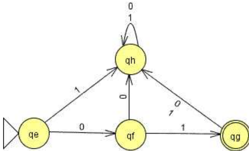
Figure 9: A DFA which accepts only the string 01.
