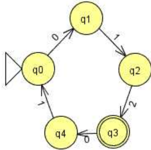
Figure 17: An NFA which accepts 012(01012)^* .
