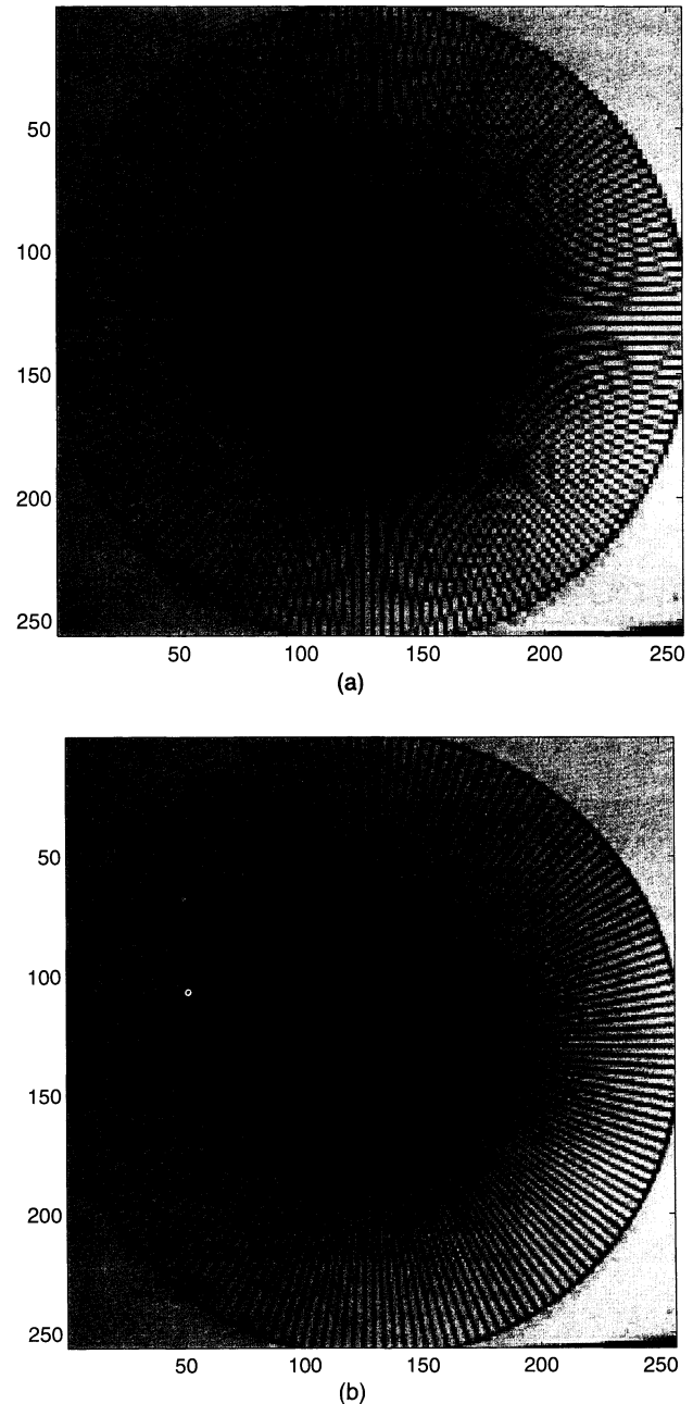
Fig. 7 Spoke-target comparison. Image (a) is a staring image, and image (b) is a level-2 microscan of the same target. Pixel replication has been applied to the staring image to facilitate a comparison.
