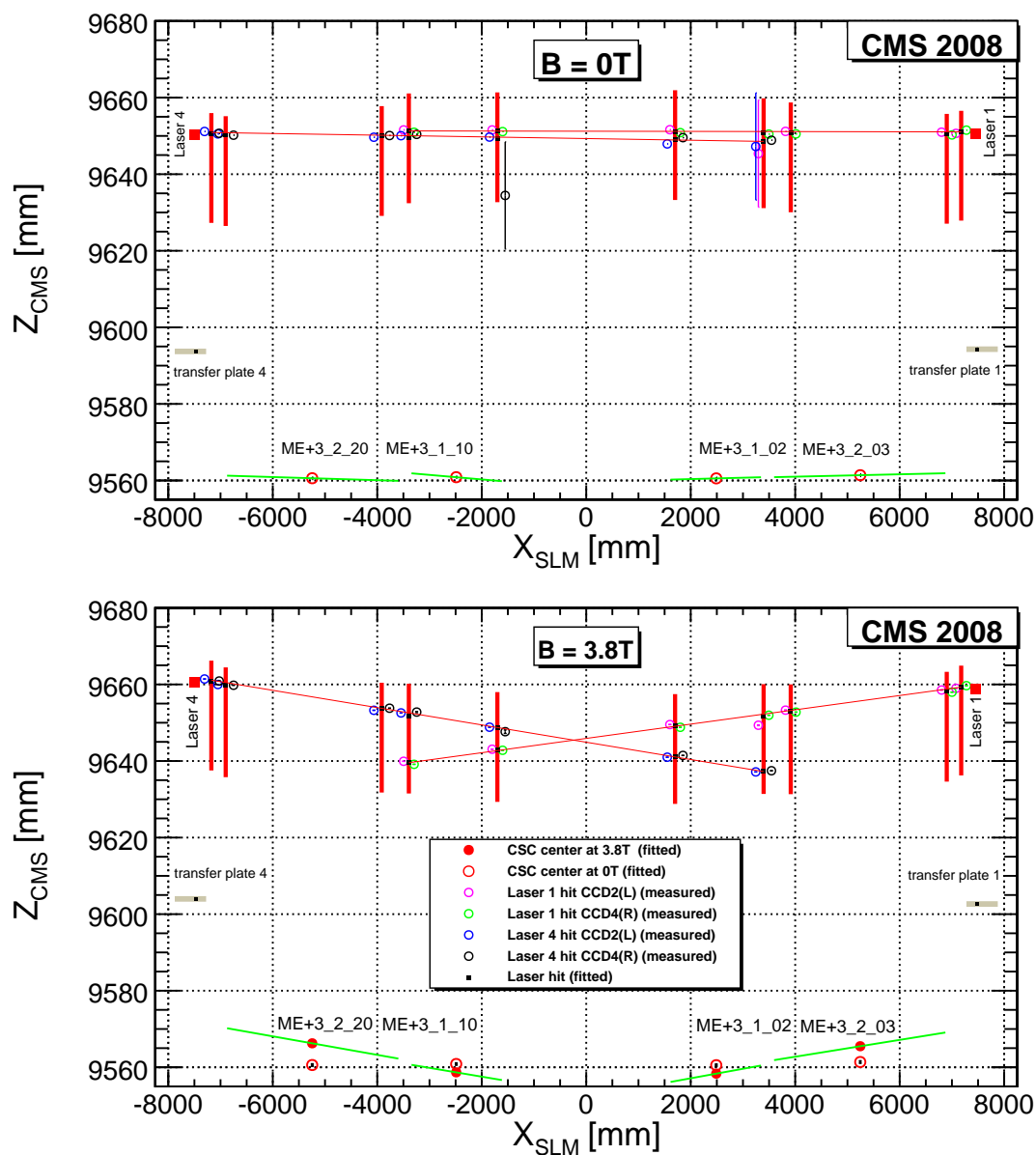
Figure 5: Reconstruction results for positions of chambers and sensors in z_{CMS} vs. their positions x_{SLM} along a straight-line monitor at B = 0\text{ T} (top) and 3.8\text{ T} (bottom). The data shown are for the straight-line monitor connecting transfer plates 1 and 4 of station ME+3. Large vertical bars indicate fitted positions of optical sensors. Laser hits on optical sensors are indicated by open circles with error bars on hit positions smaller than marker symbols. Long near-horizontal lines represent fitted laser beams. Reconstructed CSC chamber tilts are indicated by the short near-horizontal lines.
