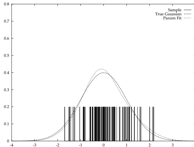
Figure 2.4: Three views of a Gaussian density with a mean of 0.0 and a variance 1.0: First a sample of 100 points drawn from the density. Each point is represented a vertical black line. Second the density of the true Gaussian. Third the Parzen density estimate constructed from the sample. The window functions are Gaussians with variance 0.35.
