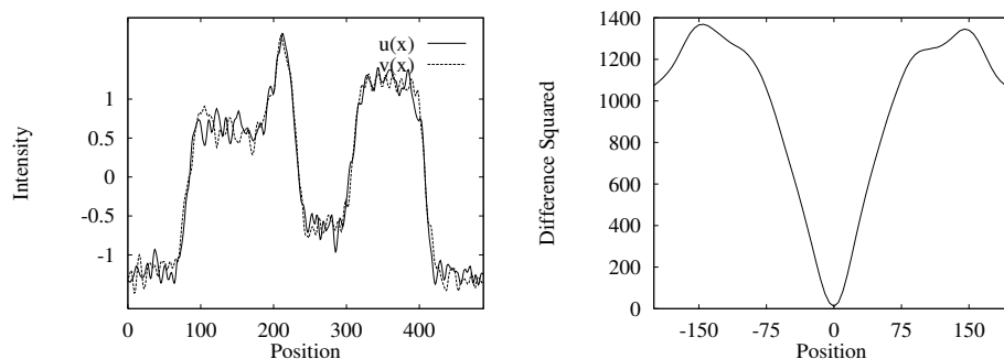
Figure 4.3: On the left is a plot of image and model that are identical except for noise. On the right is a plot of C(T) versus translation. There is a significant minimum at the correct aligning translation of 0 pixels.
