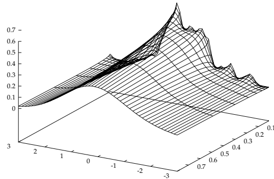
Figure 2.8: A parametric surface plot of the Parzen density versus variance (this is the same data shown in the previous graph). The horizontal and vertical axes are the location and density respectively. Variance changes with depth in the graph. Here variance ranges from 0.80 to 0.01.
