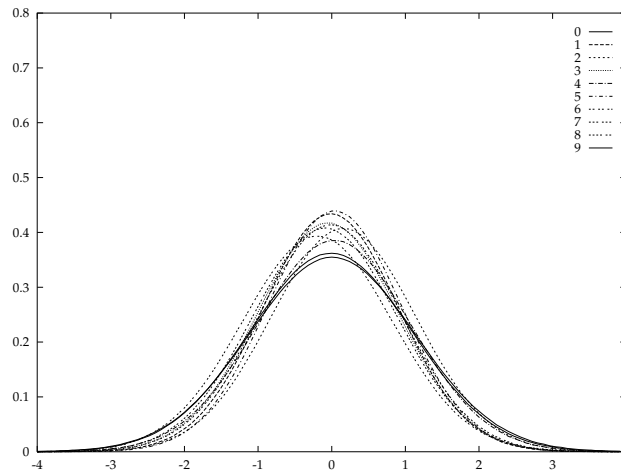
Figure 2.2: The maximum likelihood density estimates for ten different samples of 100 points drawn from the same Gaussian.
