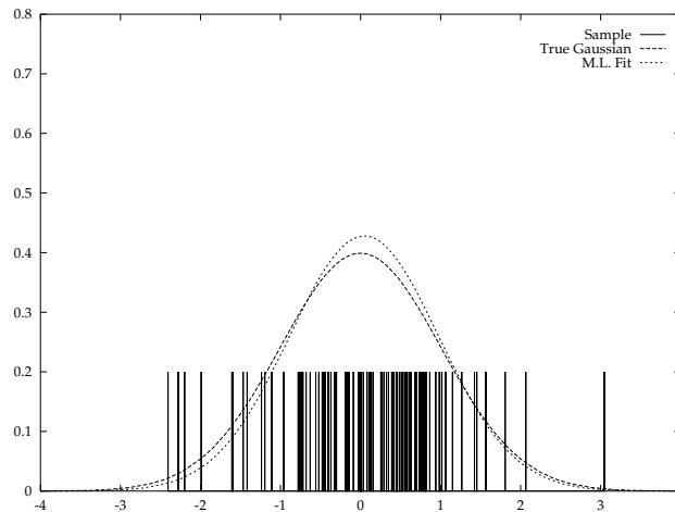
Figure 2.1: Three views of a Gaussian density with a mean of 0.0 and a variance 1.0: First a sample of 100 points drawn from the density. Each point is represented a vertical black line. Second the density of the true Gaussian. Third the density of the Gaussian estimated from the sample (mean = 0.045, variance = 0.869).
