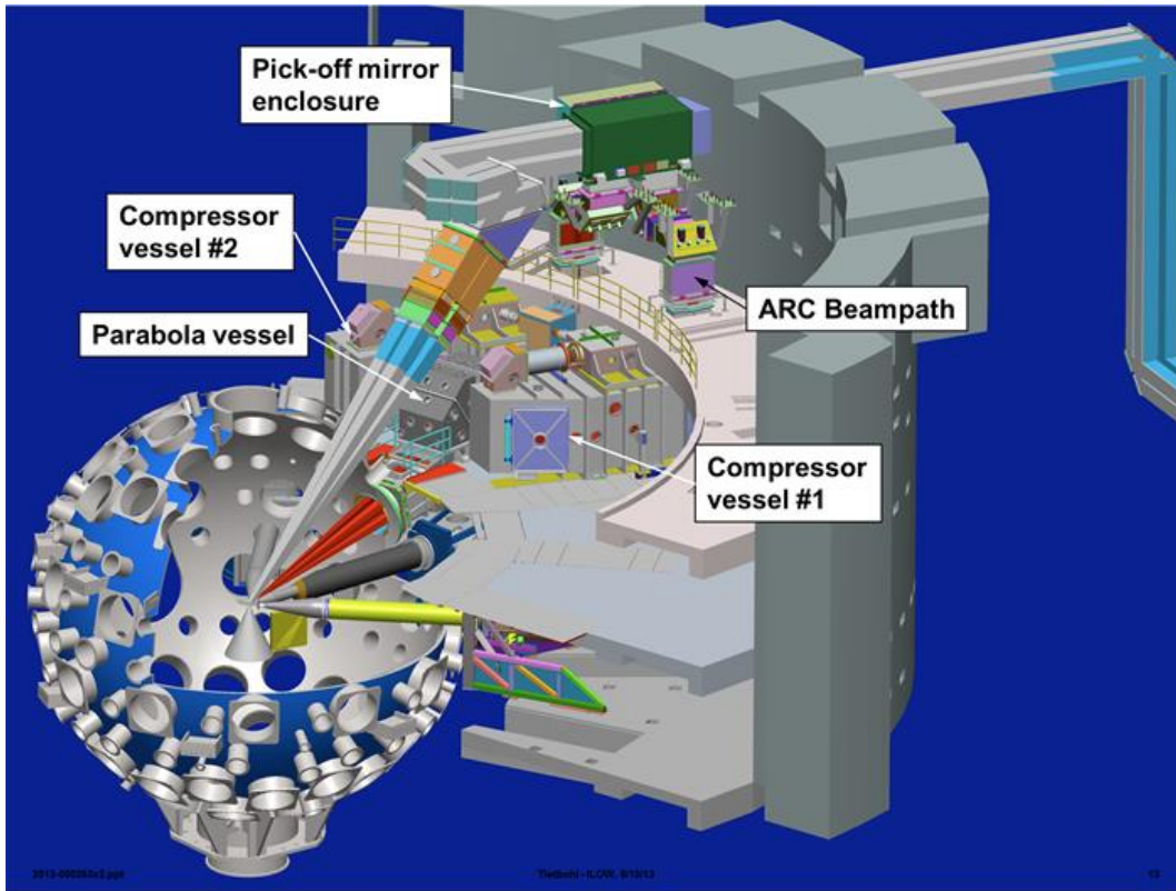
Figure 1.0 Schematic view of some of the elements in the National Ignition Facility, where ARC beams, after amplification in the NIF laser, are compressed in the target bay and focused to target chamber center (TCC). For a sense of scale in this figure, the round TCC in the lower left is 10 meters in diameter.
