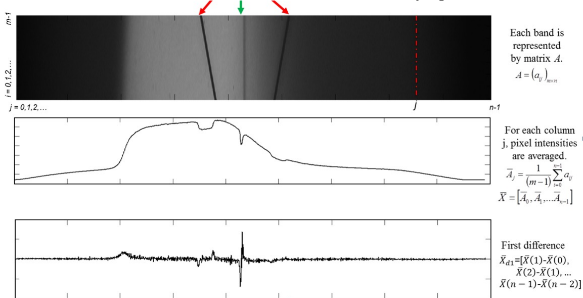
Figure 4.2.2 Example of the crosshairs algorithm locating a lower contrast line in the presence of competing lines. The band (top) is compressed to form a (middle) signal and then processed (below) to emphasize the higher slope of the vertical line. Low-contrast lines (top middle arrow) can be discriminated from high-contrast, off-angle lines (top left/right arrows).
