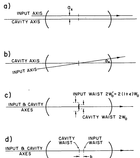
Fig. 2. Possible misalignments of the input axis with respect to the cavity axis: (a) transverse displacement in the x direction; (b) tilt through an angle \alpha_x ; (c) waist size mismatch; and (d) axial waist displacement. Equivalent to (a) and (b) are transverse displacements and tilts in the y dimension.
