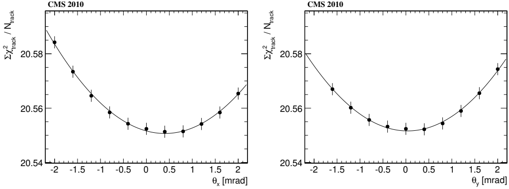
Figure 3. Dependence of the total \chi^2 of the track fits, divided by the number of tracks, on the assumed \theta_x (left) and \theta_y (right) tilt angles for |\eta| < 2.5 and p_T > 1 \text{ GeV}/c . The error bars are purely statistical and correlated point-to-point because the same tracks are used for each point.
