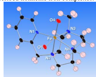
Figure 1. Left, schematic representation of the ligand. Right, thermal ellipsoid plot (50% probability) of 1 ; triflate ligands (except for the O atoms bound to Fe) omitted for clarity.
