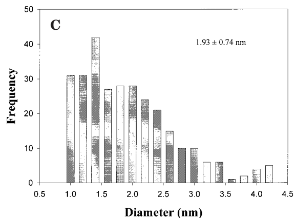
Figure 1. Representative TEM micrographs (A and B) of fresh CuC6 (rt, 3 \times ) particles synthesized with superhydride as the reducing reagent. Scale bars are 51 nm. (C) depicts the particle size histogram.
