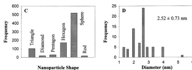
Figure 3. Representative TEM micrographs (A and B) of CuC6 (rt, 3 \times ) particles after prolonged low-temperature thermal annealing. Scale bars (A) 100 nm and (B) 33 nm. (C) depicts the population distribution of particles of varied shapes. (D) shows the size histogram of the small particles exhibited in the background of (A) and (B).
