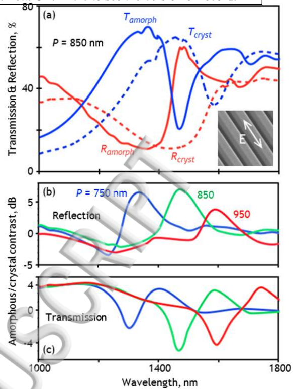
Figure 3. (a) Microspectrophotometrically measured TE-mode reflectivity and transmission spectra for the as-deposited amorphous and laser-annealed [partially] crystalline phases of a 300 nm thick GST nano-grating metamaterial with a period P = 850 nm [slot width s = 130 nm]. (b, c) Spectral dispersion of TE-mode reflection (b) and transmission (c) switching contrast, evaluated as 10\log(A/C) where A and C are respectively the amorphous and crystalline levels, for a selection of GST nano-grating periods [as labelled].
