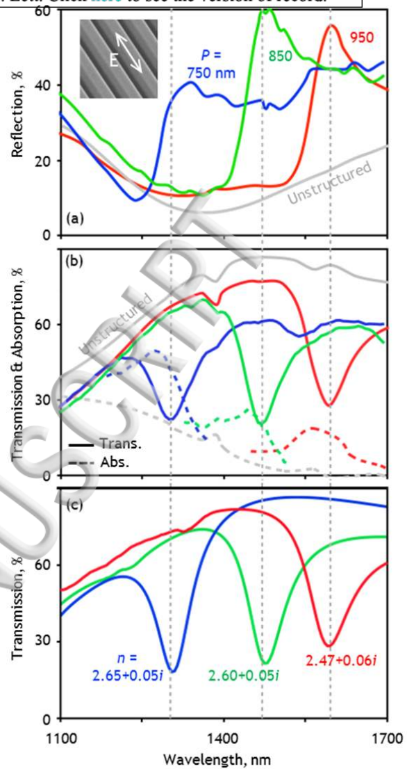
Figure 2. (a, b) Microspectrophotometrically measured Reflection R , transmission T and absorption A [ =1-(R+T) ] spectra for 300 nm thick amorphous GST nano-grating metasurfaces with a selection of periods P [as labelled; slot width s = 130 nm], under TE-polarized illumination, alongside spectra for the unstructured amorphous GST film. (c) Numerically simulated transmission spectra calculated using a non-dispersive GST refractive index value for each grating period [as labelled] selected to reproduce experimental resonance positions and widths.
