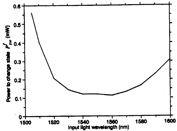
Fig. 9. Input power required to change flip-flop state versus wavelength.
