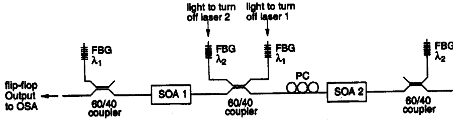
Fig. 5. Implementation of flip-flop. Each component laser is formed by a SOA and two FBGs.
